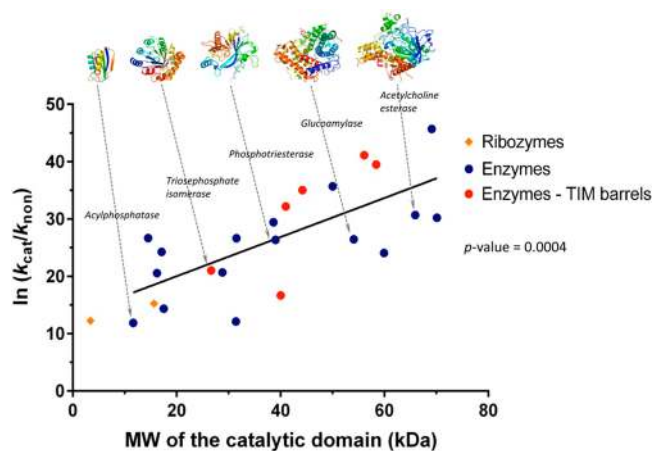
Figure 3. Molecular weight of the catalytic domain of an enzyme versus the observed rate enhancement, \ln(k_{\text{cat}}/k_{\text{uncat}}) . Selected structures for the catalytic domains are illustrated across the top of the graph and labeled (arrows point to the corresponding point on the graph). Ribozymes are shown with orange diamonds and enzymes are shown with filled circles. The TIM-domain enzymes are shown in red. A linear regression is also shown ( y = 0.34x + 13.3 , R^2 = 0.48 ). Values are taken from references detailed in Table S1.
