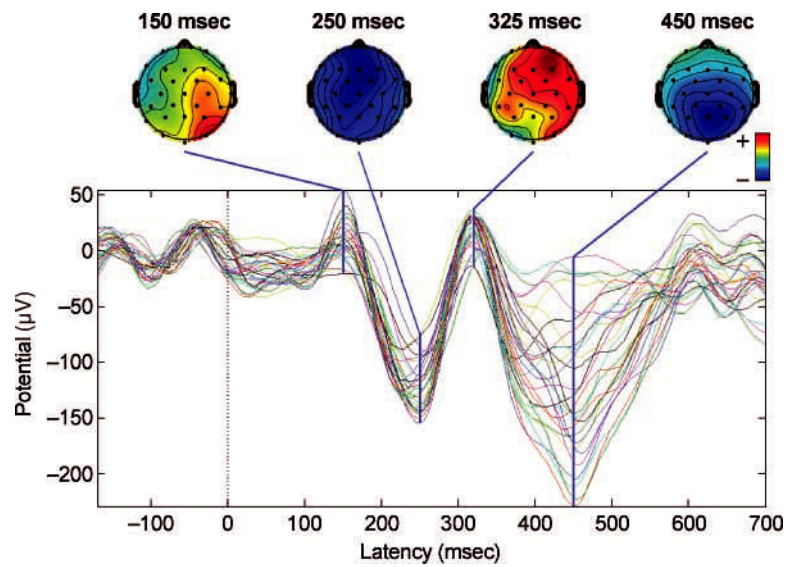
Figure 5. (Top) Voltage maps centered on the four primary measurement epochs. These were formed from difference waves (bottom) calculated by subtracting the full repetition from the unrelated condition.
