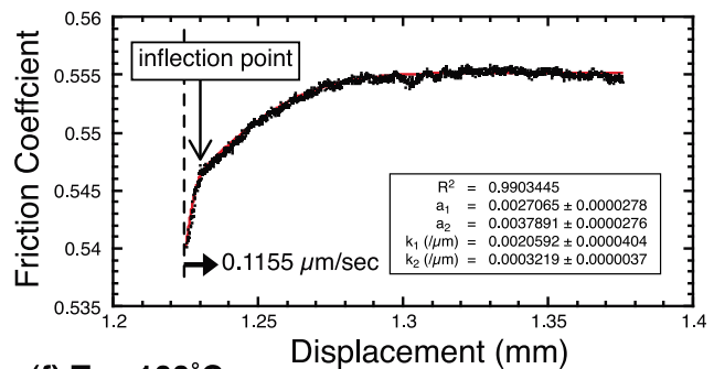
(f) T = 100^\circ\text{C}
