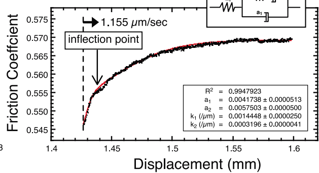
(b) T = 400^\circ\text{C}
