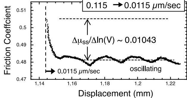
Figure 7. Plots of change in friction coefficient (a, b) for V = MV (stepwise increase in V from 0.115 to 1.155 \mu\text{m/s} ) and (c–e) at V = LV (stepwise increase in V from 0.0115 to 0.115 \mu\text{m/s} ). The flow law was used for curve fitting in Figures 7a–7e. With increasing T , the inflection point became distinct because a_2 increased relative to a_1 . (f) Example of stepwise decrease of V from 0.115 to 0.0115 \mu\text{m/s} at T = 100^\circ\text{C} . Continuous oscillations developed in several of the results for LV conditions (Figure 3c).
