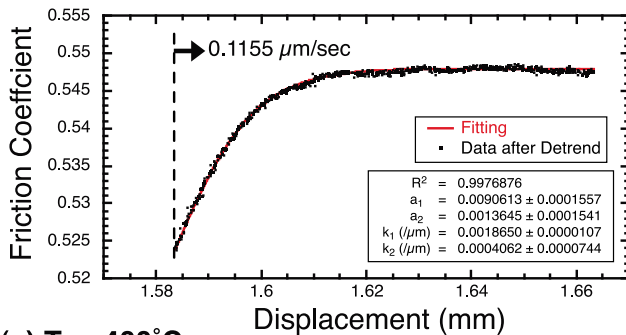
(e) T = 400^\circ\text{C}
