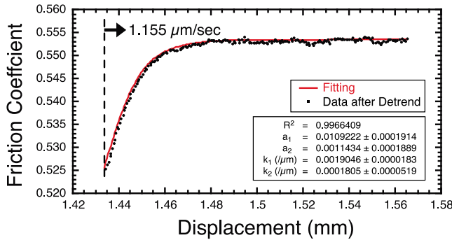
(a) T = 100^\circ\text{C}
