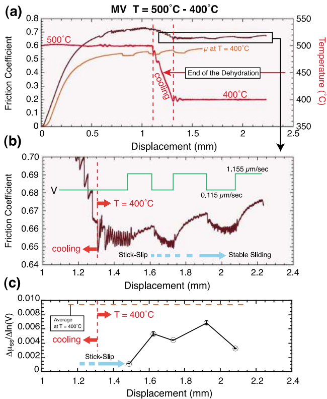
Figure 14. Influence of newly formed forsterite on strength and frictional behaviors during shearing. (a) During shearing, the specimen was cooled at 3.3^{\circ}\text{C}/\text{min} at d = 1.1 mm from T = 500^{\circ}\text{C} , where dehydration took place, to 400^{\circ}\text{C} , where, under MV conditions, dehydration ceased. After cooling toward 400^{\circ}\text{C} , the friction coefficient (brown line) did not stabilize at the same level as its value at T = 400^{\circ}\text{C} (orange line), although it did decrease slightly during cooling. (b) Stick-slip behavior at T = 500^{\circ}\text{C} did not cease immediately after stopping the dehydration but rather diminished gradually, and (c) velocity-dependence became positive with each stepwise change in velocity.
