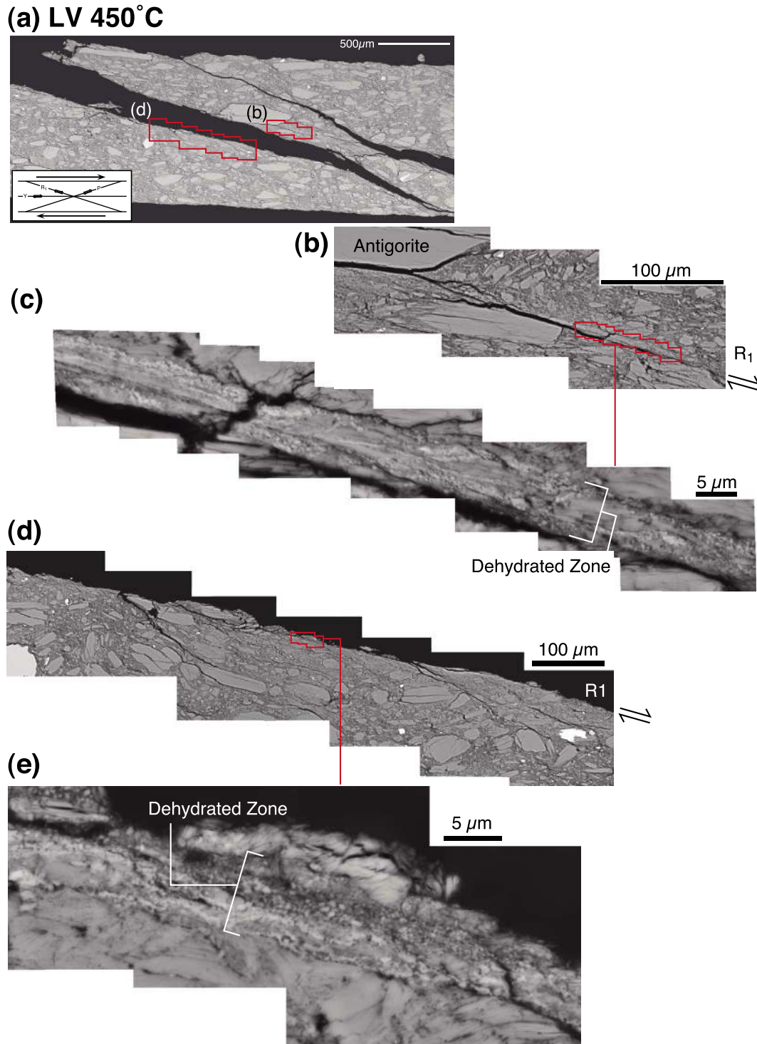
Figure 13. (a) Backscattered-electron SEM images for an experimental product that exhibited stick-slip behavior (Figure 2c) at (T, V) = (450^{\circ}\text{C}, \text{LV}) and contained a small amount of forsterite (Figure 10d). Shearing was dextral. These images demonstrate that dehydration took place only in sheared zones. (b, d) Magnified images showing bright, fine forsterite particles along R_1 shears. (c) Forsterite particles developed along antigorite cleavages in dehydration zones about 5\ \mu\text{m} thick. (e) Several narrow zones ( \sim 10\ \mu\text{m} thick) containing numerous submicron-sized forsterite particles are concentrated along an R_1 shear.
