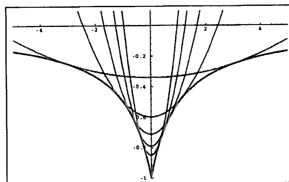
\inf_{z \geq 0} E(x, \sigma, z)
