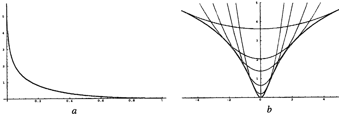
Figure 11. Lorentzian outlier process: (a) Penalty function, (b) inimum of E(x, z, \sigma) .
