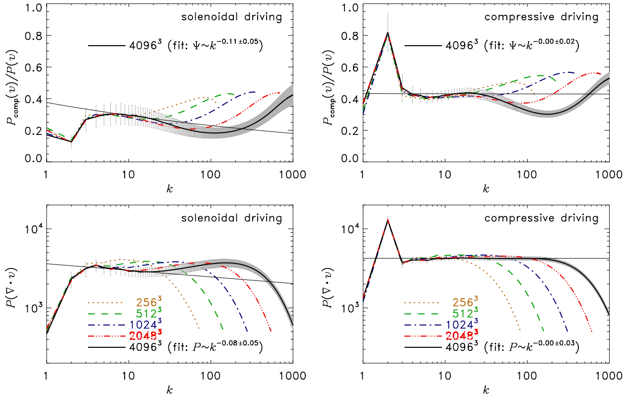
Figure 8. As Fig. 6, but showing Fourier power spectra of the compressive ratio defined in equation (12) (top panels) and of \nabla \cdot \mathbf{v} (bottom panels) for solenoidal driving (left-hand column) and compressive driving (right-hand column). \Psi and P(\nabla \cdot \mathbf{v}) decrease for solenoidal driving, but stay remarkably constant for compressive driving in the inertial range.
