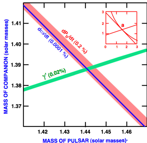
Fig. 1. Concordance between observations and the post-Newtonian predictions of general relativity for the binary pulsar PSR 1913+16. Inset shows the full m_1 - m_2 plane and the intersection region “a.” The width of each band reflects the error in measuring each parameter.
