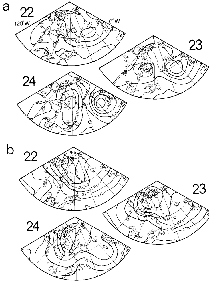
Figure 7. The 1000 mb geopotential (a) and 700 mb temperature (b) for the period 22–24 September 1982 and the region 40^{\circ}\text{N} – 90^{\circ}\text{N} and 120^{\circ}\text{W} – 0^{\circ}\text{W} corresponding to that shown in Figs. 5 and 6. The contour intervals are 60 m and 5 K, respectively.
