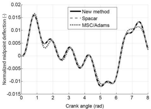
Fig. 7 Mid-point deformation of the connector compared with Spacar and MSC/Adams. Figure was made using Matlab for plotting and Adobe Illustrator for labels
