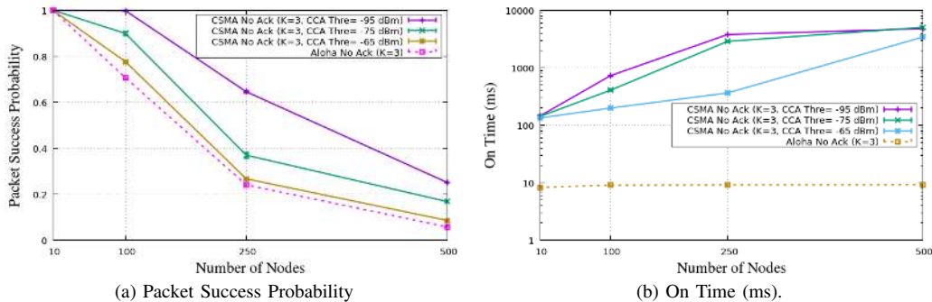
Fig. 1. CSMA and Aloha packet success ratio and ON time.
