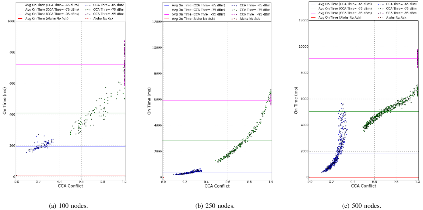
Fig. 3. Node energy consumption and CCA conflict rate for different CCA threshold values, and for Aloha.
