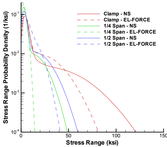
Figure 15: Dirlik stress range PDFs of EL-FORCE response at 0.9216 lb/in load.
