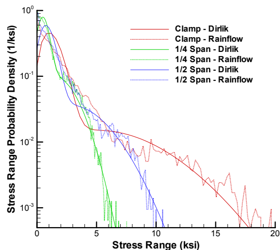
Figure 10: Stress range PDFs of nonlinear response prediction at 0.1152 lb/in load.
