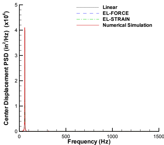
Figure 3: Center displacement response due to 7.2 \times 10^{-3} lb/in load, on a linear scale.
