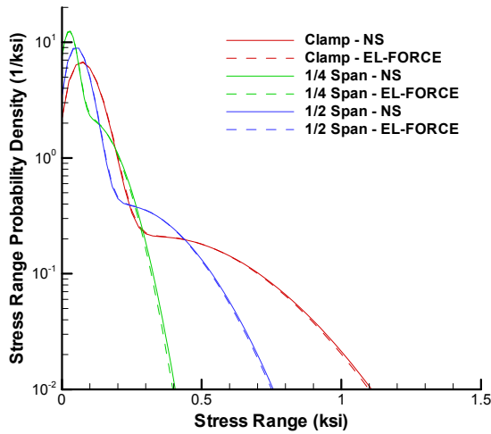
Figure 13: Dirlik stress range PDFs of EL-FORCE response at 7.2 \times 10^{-3} lb/in load.
