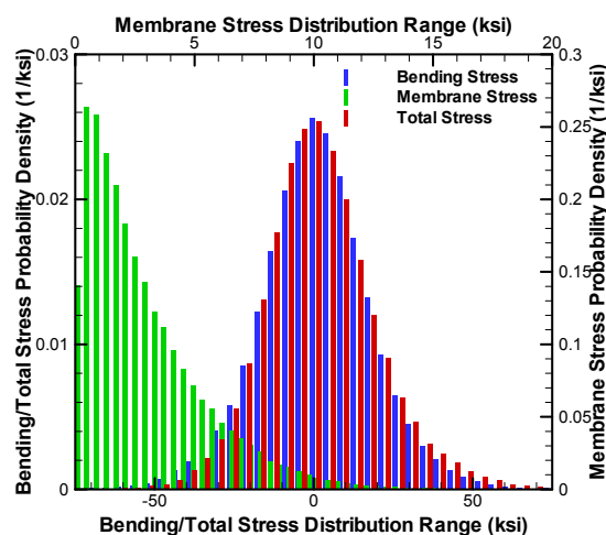
Figure 12: Nonlinear stress PDF at clamped end for 0.9216 lb/in load.
