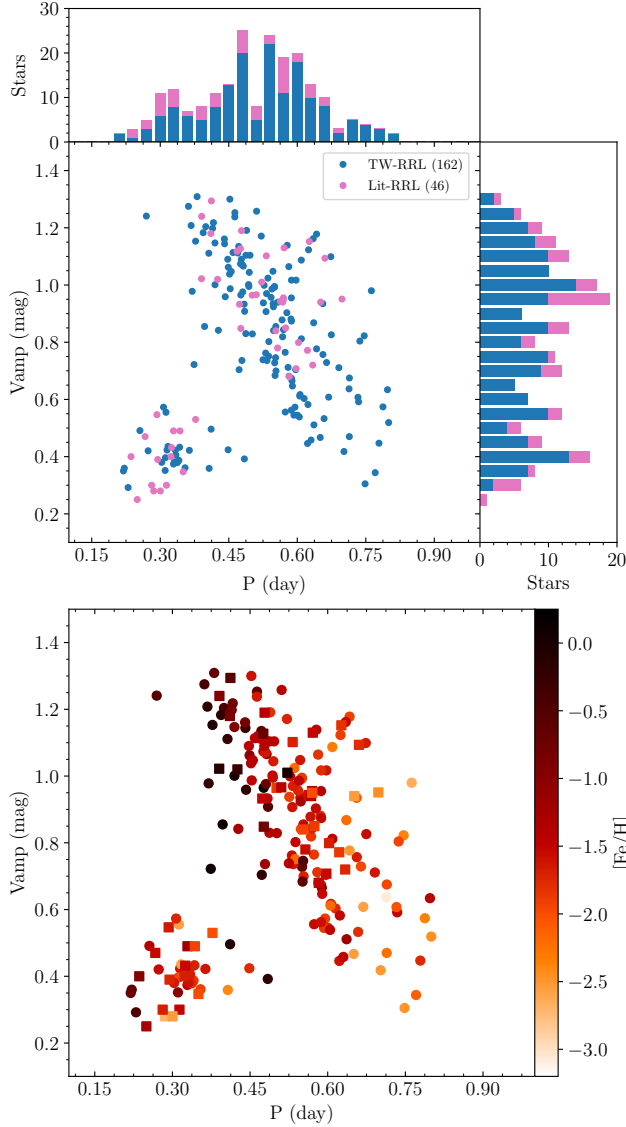
Figure 4. Top: Bailey diagram for the TW-RRL sample (blue), and the Lit-RRL sample (pink). The top and left histograms show the distribution of period and V-band amplitudes, respectively. Bottom: Bailey diagram colored by metallicity according to the color bar on the right. The TW-RRL and the Lit-RRL stars are marked with circles and squares, respectively.
