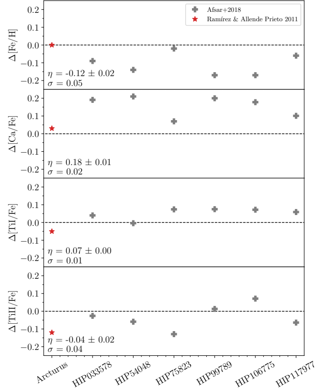
Figure 3. Difference between the iron and \alpha -element abundances derived in this work and those of Afşar et al. (2018) for a sample of six HB stars, shown as grey crosses. The median ( \eta ) and median absolute deviation ( \sigma ) of the difference is shown in each panel. A red star shows the same difference for Arcturus (Ramírez & Allende Prieto 2011).
