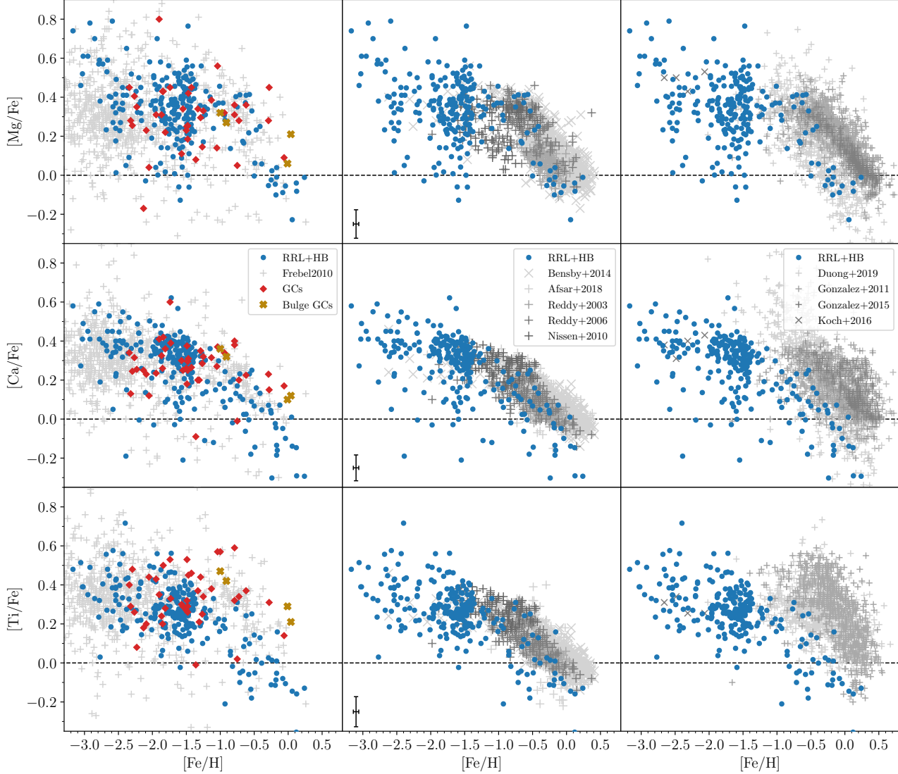
Figure 6. Abundances of Mg, Ca, and Ti for the RRL+HB sample, compared to three typical Galactic populations. Left: Globular clusters and Halo field stars. Middle: Thin and thick disk field stars. Right: Bulge field stars. References – GCs: Pritzl et al. (2005); Carretta et al. (2009a,b, 2010a), Bulge GCs: Gonzalez et al. (2011), The remaining references are labeled according to the first author and year of publication: Frebel (2010), Bensby et al. (2014), Reddy et al. (2003), Reddy et al. (2006), Afşar et al. (2018), Nissen & Schuster (2010), Duong et al. (2019), Gonzalez et al. (2011), Gonzalez et al. (2015), Koch et al. (2016).
