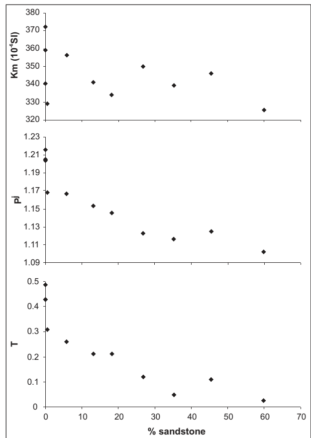
Figure 4: Variation of magnetic susceptibility ( K_m ), corrected degree of anisotropy ( P_j ) and shape parameter ( T ) with changing amount of sandstone within distal turbidite deposits of the Upper Ordovician Ittre Formation. Note that whereas a relationship does come forward in the case of P_j and T , there is no clear relationship in the case of K_m . See text.
