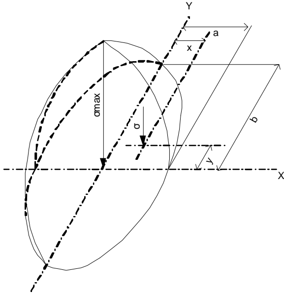
Fig. 3: Compressive stresses in an elliptical contact area
