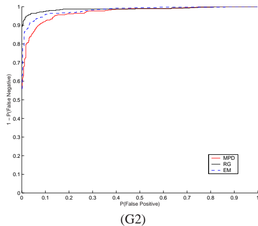
Figure 5. ROC curves for G1 and G2: 'MPD' stands for Minimum Pair Distance, 'EM' for Eyes and Mouth, 'RG' for Regular Grid.
