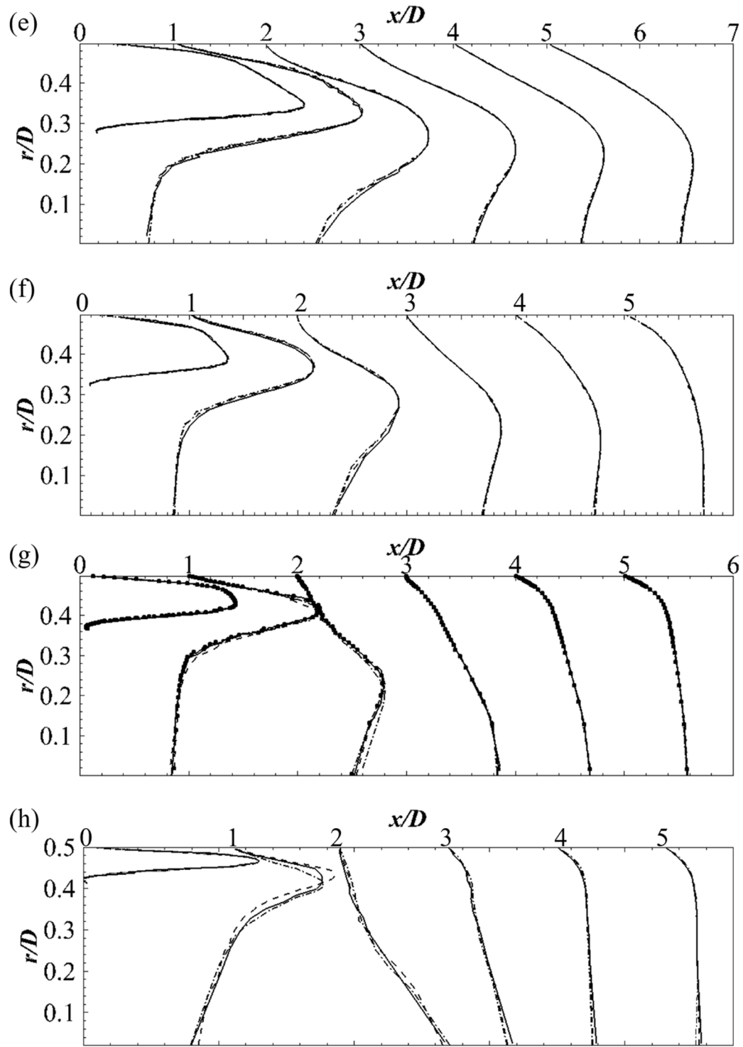
Figure 36 Azimuthal- and time-averaged streamwise profiles at the streamwise locations of x/d = 0.2, 1, 2, 3, 4, 5 in the wake flow behind the sphere for different grid resolutions: Case 1: Solid lines; Case 2: Dashed; Case 3: Dash-dotted; Case 4: Black circles with BR = (a) 0.1; (b) 0.2; (c) 0.4; (d) 0.5; (e) 0.6; (f) 0.7; (g) 0.8; (h) 0.9
