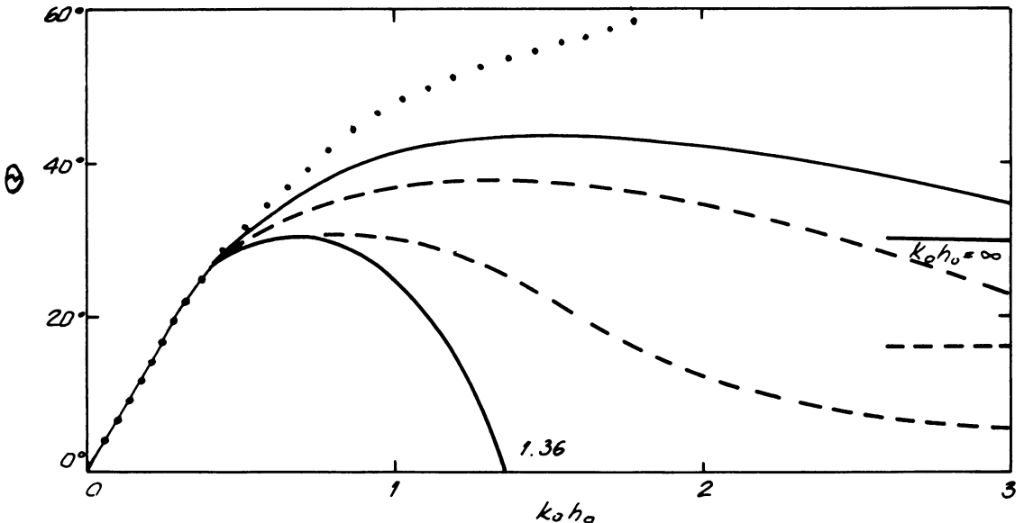
FIG. 1. Stability plot for water waves according to Hayes (solid lines) and BII (broken lines). Differences only become visible for h_0 k_0 > \frac{1}{2} , and serious for h_0 k_0 > 1 . Dots correspond to K-de V.
