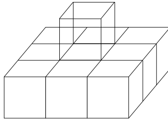
Figure 8: A polytope which can be tiled by 3d -dominoes but all of whose sides are odd.
