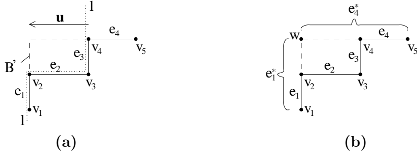
Figure 6: Transforming the turn sequence of the polygon.
