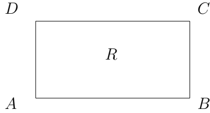
Figure 2: A G -rectangle R with vertices A, B, C, D .
