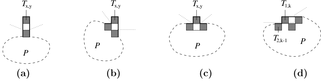
Figure 3: The four cases considered in the proof of Lemma 3.2.
