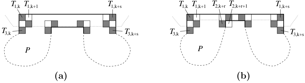
Figure 4: Two subcases in the proof of Lemma 3.2.
