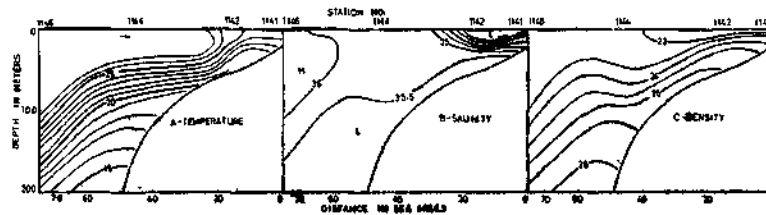
Fig. 7. Vertical distribution of hydrographic parameters in the region off Karwar.
