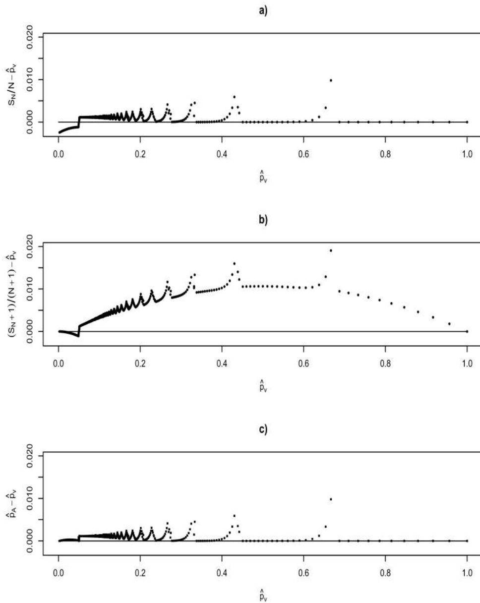
Figure 6. Validity of simple p-value estimators for the truncated SPRT with m = 9999 , p_a = .04 and p_0 = .0614 with \alpha_0 = \beta_0 = .0001 . Figure 6a shows S_N = N - \hat{p}_v vs. \hat{p}_v , and Figure 6b shows (S_N + 1)/(N + 1) - \hat{p}_v vs. \hat{p}_v . Figure 6c shows \hat{p}_A - \hat{p}_v vs. \hat{p}_v , where \hat{p}_A is defined by (9). In both Figures 6a and 6b the difference falls below the line at 0, while in Figure 6c the difference never falls below 0, therefore, \hat{p}_A is the only valid p-value of the three.
