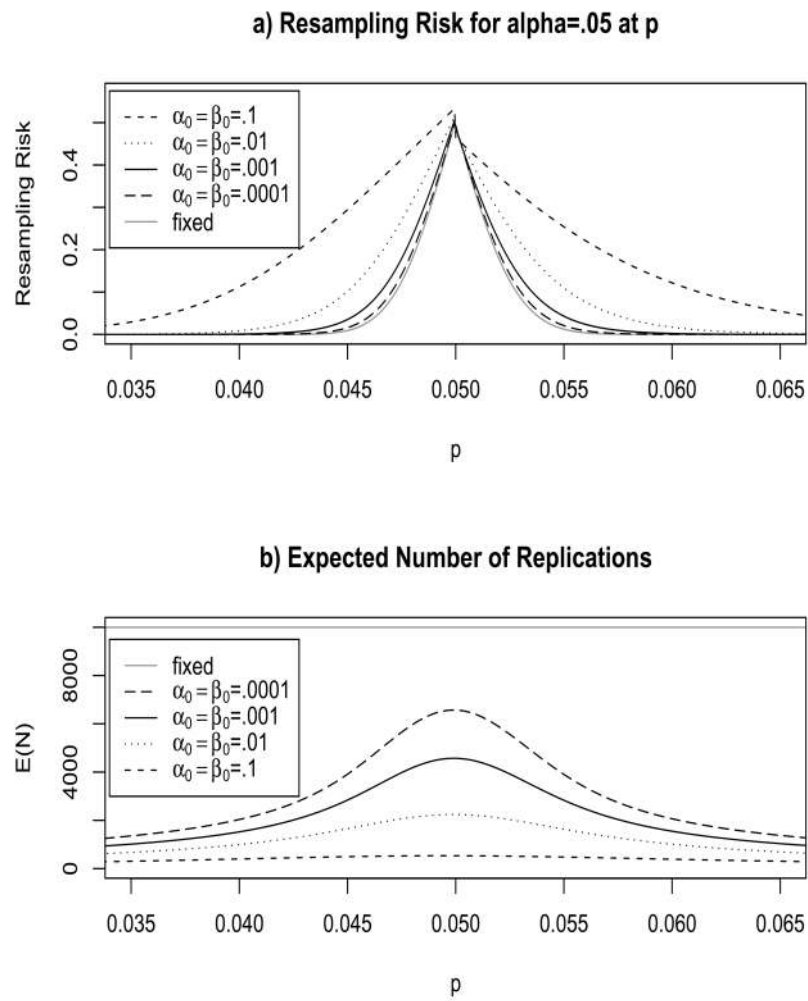
Figure 4. Properties of truncated SPRT with m = 9999 , p_a = .04 and p_0 = .0614 (so that C_0 = .05 ) using the Wald boundaries with \alpha_0 and \beta_0 both equal to either 0.1, 0.01, 0.001, or 0.0001 (this corresponds to the parametrizations with C_1 = -C_2 equal to either 4.862, 10.168, 15.283 or 20.380 respectively). Figure 4a is RR_{.05}(p) and Figure 4b is E(N) , where both are calculated exactly using the algorithm in the appendix.
