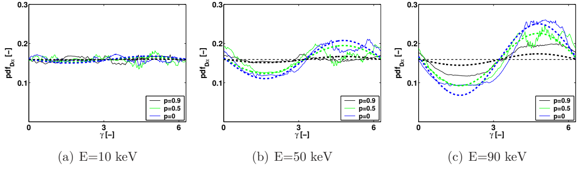
Figure 10. Comparison of \text{pdf}_{D\alpha} as computed with FIDASIM with the cosine model \text{pdf}_{D\alpha} (equation 52) at various positions in velocity space. The thick dashed lines are the model cosine, and the thin dashed line is the uniform distribution.
