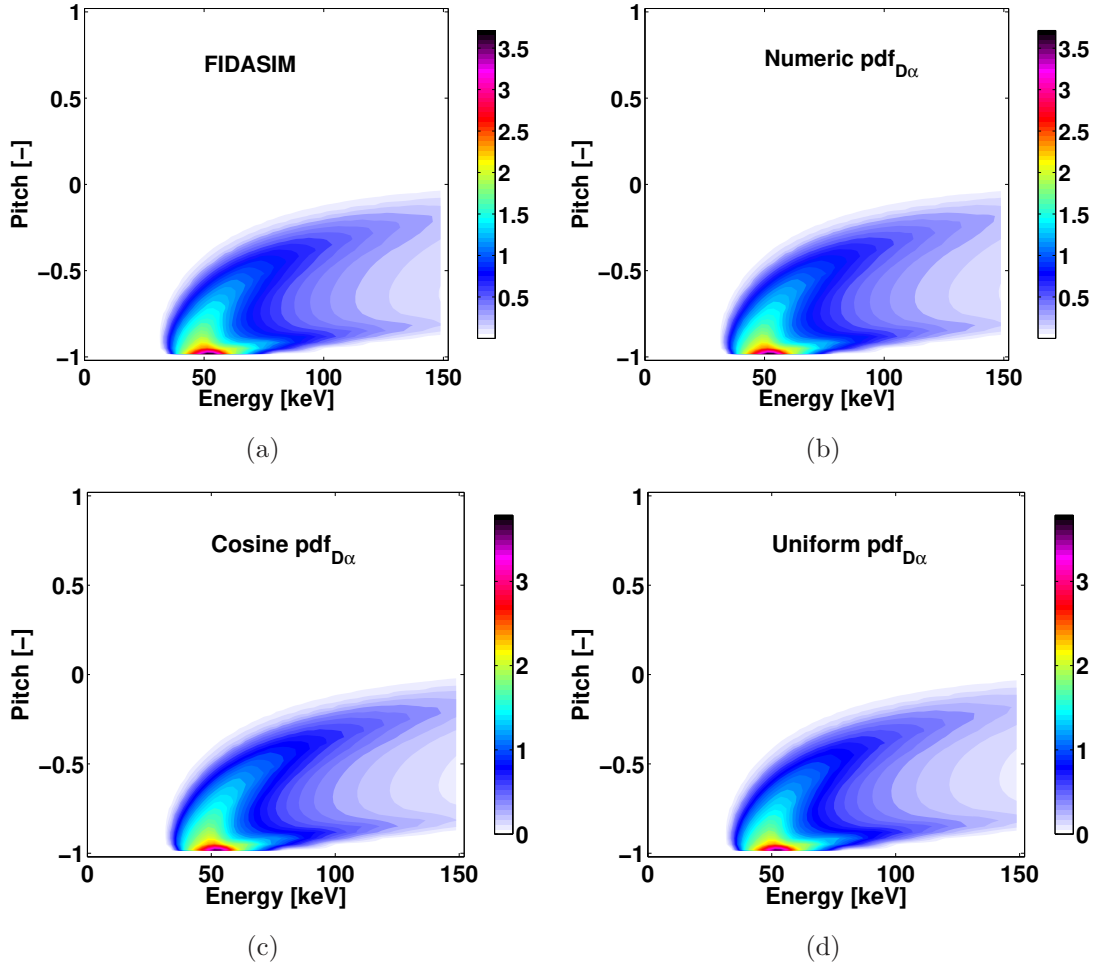
Figure 12. Full FIDA weight functions as computed with (a) traditional FIDASIM, (b) equation 56 for numerically computed \text{pdf}_{D\alpha} using FIDASIM, (c) equation 56 for the cosine model \text{pdf}_{D\alpha} , (d) equation 56 for the uniform model \text{pdf}_{D\alpha} . The projection angle is \phi = 155^\circ . The wavelength range is 660-661 nm. The magnetic field is 1.74 T.
