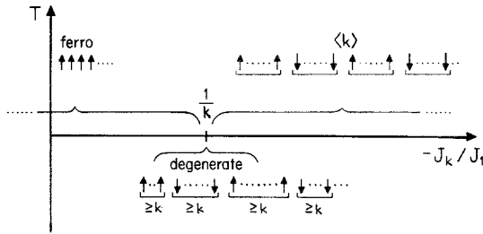
Fig. 1. The zero temperature phase diagram for the system described by the model Hamiltonian of Eq. (1). The three ordered phases that occur are indicated schematically.
