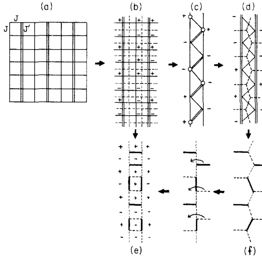
Fig. 2. (a) The PUD model: The single and double bonds represent ferromagnetic interactions J , and antiferromagnetic interactions J' , respectively. (b) A section of the PUD model with the dual lattice shown dashed. The + and - signs indicate the spins in a typical ground state for |J'| > J . The antiferromagnetic vertical chains order “in phase,” in one of two possible states. On the other hand, there is a large degeneracy associated with the possible states of the vertical ferromagnetic chains. (c) Under the transformation s_i \rightarrow t_i t_{i+1} , the vertical ferromagnetic chain in (b) maps into a chain with alternating nearest-neighbor interactions (zig-zags), and ferromagnetic second-neighbor interactions (vertical). The + and - signs now indicate the signs of the new spin variables t_i . These are defined only up to an overall sign; consequently there is a two-to-one correspondence between the ground states of the RS model and a ferromagnetic chain in the PUD model. The open circles indicate the spins to be redefined in order to map the Ising chain to the RS model through a gauge transformation. (d) The RS model, with ferromagnetic nearest-neighbor interactions, and antiferromagnetic second-neighbor interactions. The + and - signs indicate the spin states obtained after the gauge transformation from (c). Shown dashed is the dual lattice. (e) The dual ladder of the PUD model and the spins states of the original lattice from (b). The close-packed dimer configurations that are derived from this spin state are indicated by the full lines. (f) The dual of the RS model with the close-packed dimer configuration corresponding to the spin state of (d). From this dimer configuration we can obtain the geometrically equivalent configuration (e) as follows: First we “straighten out” the dual lattice, and then slide alternate horizontal bonds to one side of the vertical chain. Finally, we add a second vertical dimer chain identical to the first one to obtain the dual ladder in the dimer state (e).
