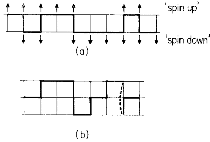
Fig. 3. (a) A directed SAW on the ladder of width two lattice spacings. Steps to the left are prohibited. At each site, we place a spin up if the walk passes through a site on the upper edge of the ladder, and vice versa for the lower edge. As the walk proceeds we trace out one of the spin configurations in the degenerate ground state of the RS model. (b) A typical SAW on a 3 \times \infty strip of the square lattice, with periodic boundary conditions. The vertical bonds directly joining the top and bottom rows are not drawn. The walk shown belongs to the class b_N as defined in the text.
