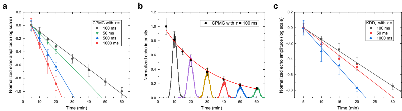
Fig. 3 Measurements of the memory lifetime. a, c Decay of the spin-wave AFC echo with the CPMG and \text{KDD}_x sequences, respectively. The two DD sequences reach their longest storage lifetime of 52.9 \pm 1.2 and 33.3 \pm 1.1 min with a period \tau = 100 ms. b The decay of the echo intensity using CPMG with \tau = 100 ms versus the storage time. Some of the single-shot oscilloscope traces of the read out signals are included. Each data point is averaged four times. The error bars indicate one standard deviation of the echo area.
