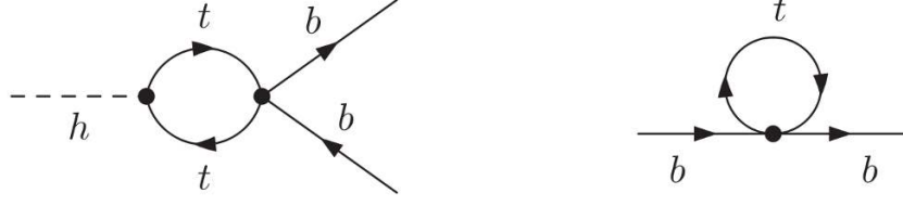
Figure 1. Examples of one-loop diagrams involving Class 8 operators to the h \rightarrow b\bar{b} process (left), and to the b -quark two-point function (right). The corresponding diagrams for h \rightarrow \tau\bar{\tau} are of similar form.
