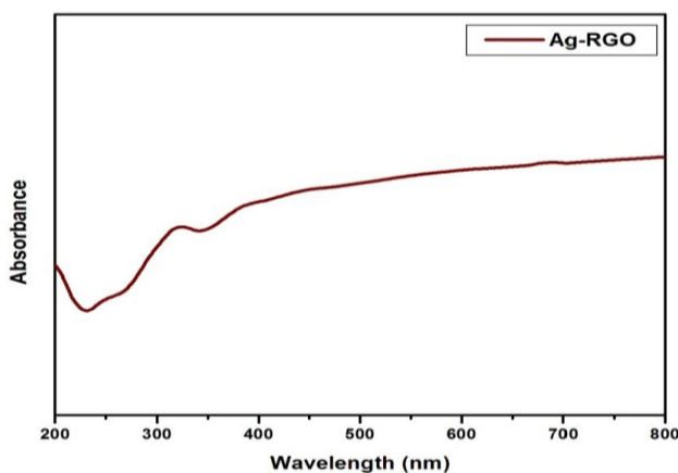
Fig. 3 Shows the UV-Vis absorption spectra of synthesized nanocomposite. UV-Vis absorption spectra of Ag-RGO nanocomposite indicated that the absorption peak of Ag nanoparticles was located at 325nm
