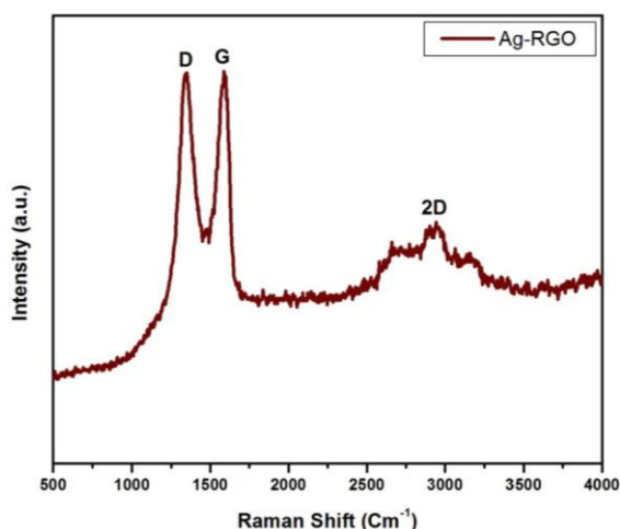
Fig.2. Raman spectra of Ag-RGO nanocomposite
