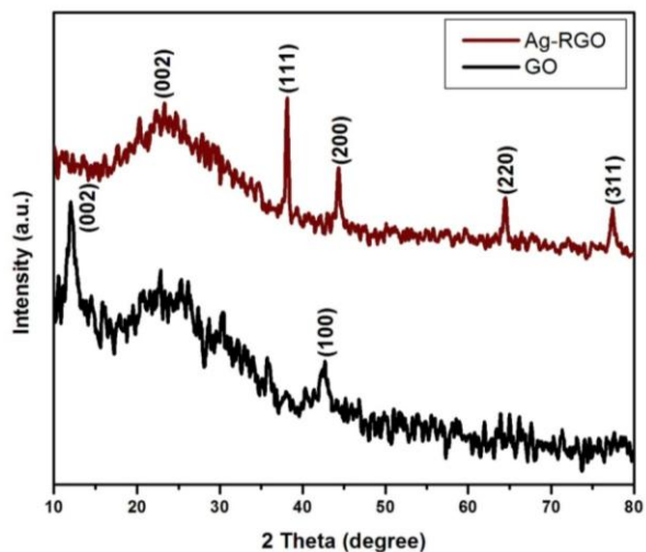
Fig.1. XRD patterns of GO and Ag-RGO nanocomposite.
