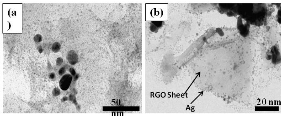
Fig. 5. HR-TEM images of Ag-RGO nanocomposite.
