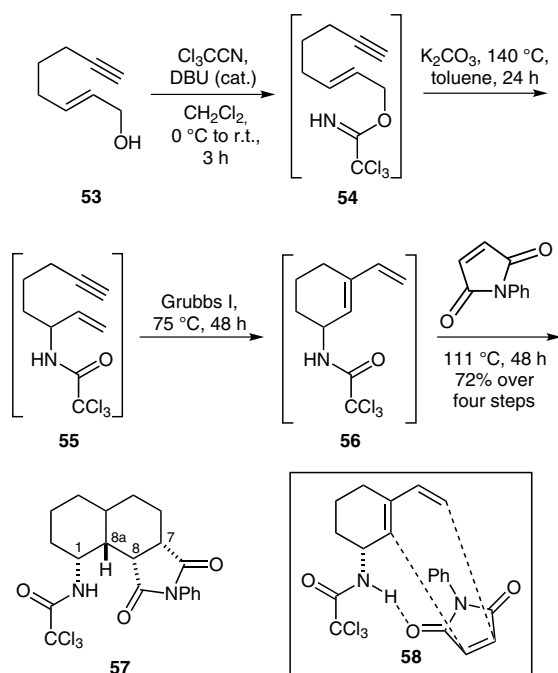
Scheme 19
