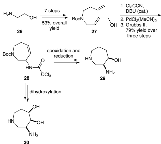
Scheme 11
