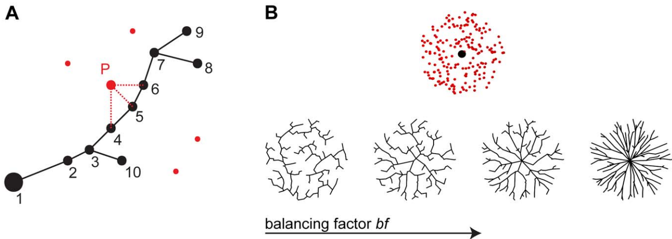
Figure 2. Generating neuronal branching structures using optimized graphs. (A) The growth described by an extended minimum spanning tree algorithm (see text). Unconnected carrier points (red) are connected one by one to the nodes of a tree (black). Red dashed lines indicate three sample Euclidean distances to the nodes of the tree for sample point P . (B) Example trees grown on homogeneously distributed random carrier points in a circular hull starting from a root located at its centre (see top). Plotted as a function of the balancing factor bf , the trees range from perfect minimum spanning trees (left) to almost direct connections from the root to any point (right). doi:10.1371/journal.pcbi.1000877.g002
