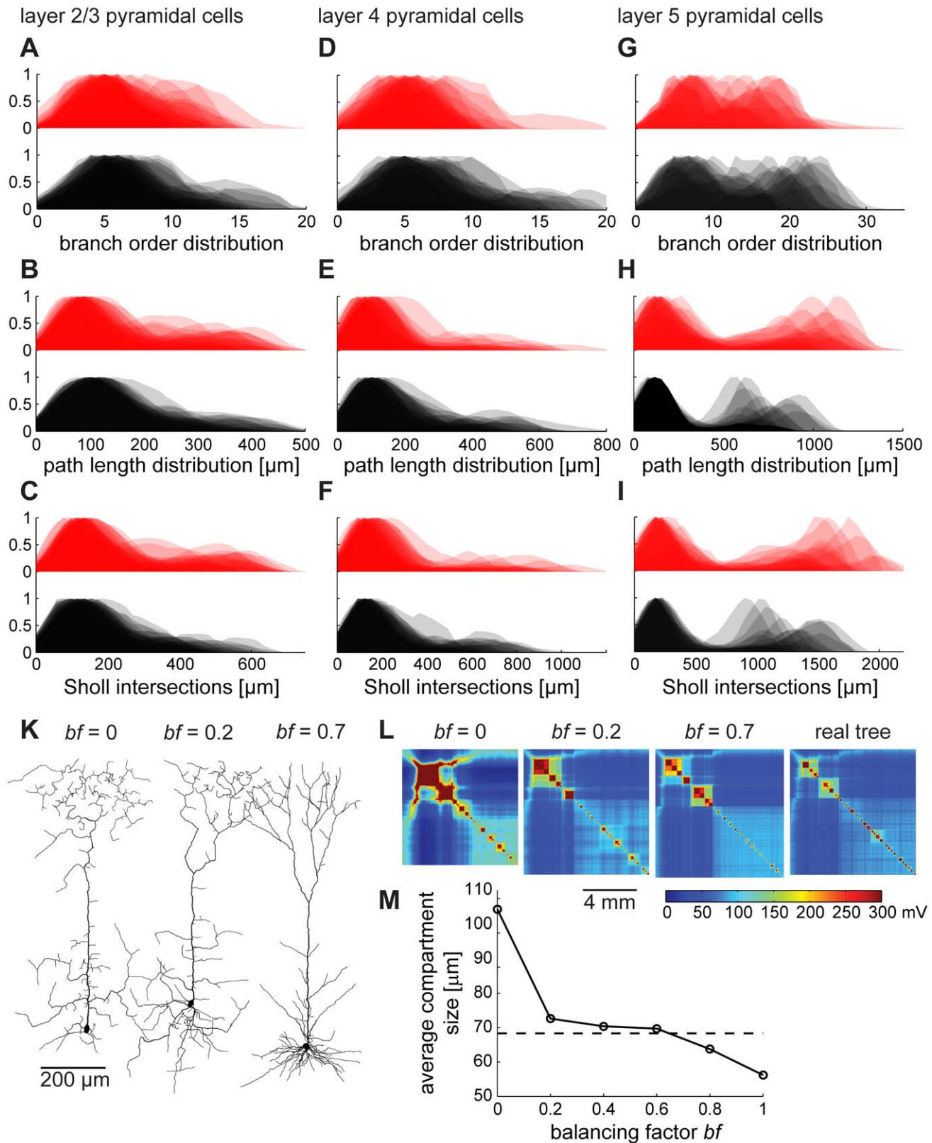
Figure 7. Validating synthetic branching structures of pyramidal cells. While branching statistics of starburst amacrine cells and hippocampal granule cells were moderately homogeneous, pyramidal cells exhibited stronger variations. Balancing factors leading to reasonable branching statistics ranged from 0.4 to 0.7. In the following we compare branching parameter distributions as in Figure 4 for synthetic (black) and original dendrites (red) of layer 2/3 (A–C), layer 4 (D–F) and layer 5 (G–I) pyramidal cells grown with a balancing factor bf=0.7 , 0.6 and 0.5 respectively. (K) Representative layer 5 pyramidal cells grown with different balancing factors bf=0 , bf=0.2 , bf=0.7 . (L) Representative electrotonic signatures of these synthetically generated dendrites and of one original layer 5 pyramidal cell for comparison. (M) Simple relationship between electrotonic compartmentalization and balancing factor. Straight line connects averages of each 100 model dendrites at different balancing factor values. Dashed line shows average compartment size of real reconstructions. doi:10.1371/journal.pcbi.1000877.g007
