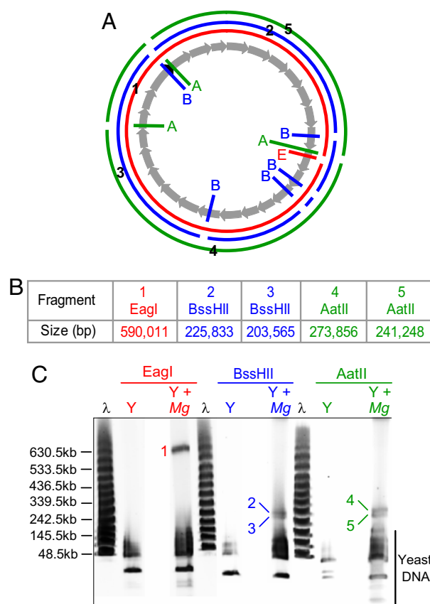
Fig. 3. Validation of an intact M. genitalium genome by restriction analysis. (A) Diagram of the EagI (red), BssHII (blue), and AatII (green) restriction fragments expected for a complete and proper assembly of the synthetic JCVI-1.1 M. genitalium genome. The 25 pieces are represented by gray arrows. (B) The sizes of the five restriction fragments indicated in (A). (C) Total DNA from clone 4 (Y + Mg) and its host strain alone (Y) were isolated from yeast cells embedded in agarose. Most of the linear DNA was electrophoresed out of the agarose plugs. These plugs were then digested with EagI , BssHII , or AatII and analyzed by FIGE on 1% agarose gels. Restriction fragments corresponding to the correct sizes are indicated by the fragment numbers shown in (A) and (B). In the lanes labeled “ \lambda ,” the lambda ladder (New England Biolabs) was loaded; sizes are indicated.
