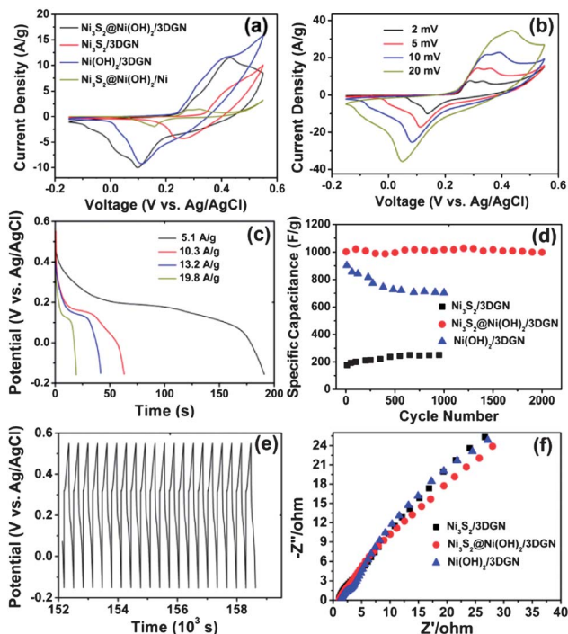
Fig. 5 (a) Cyclic voltammograms of the \text{Ni}_3\text{S}_2@(\text{Ni}(\text{OH})_2)/3\text{DGN} , \text{Ni}_3\text{S}_2/3\text{DGN} , \text{Ni}(\text{OH})_2/3\text{DGN} and \text{Ni}_3\text{S}_2@(\text{Ni}(\text{OH})_2)/\text{Ni} foam electrodes within the potential range of -0.15 to 0.55 \text{ V} at a constant scan rate of 5 \text{ mV s}^{-1} . (b) Cyclic voltammograms of the \text{Ni}_3\text{S}_2@(\text{Ni}(\text{OH})_2)/3\text{DGN} at different scan rates of 2 , 5 , 10 and 20 \text{ mV s}^{-1} . (c) Discharge curves for the \text{Ni}_3\text{S}_2@(\text{Ni}(\text{OH})_2)/3\text{DGN} at various current densities. (d) Cycling stability of the \text{Ni}_3\text{S}_2/3\text{DGN} , \text{Ni}_3\text{S}_2@(\text{Ni}(\text{OH})_2)/3\text{DGN} and \text{Ni}(\text{OH})_2/3\text{DGN} at a current density of 5.9 \text{ A g}^{-1} . (e) The last 20 charge–discharge curves for the \text{Ni}_3\text{S}_2@(\text{Ni}(\text{OH})_2)/3\text{DGN} . (f) Nyquist plots of the \text{Ni}_3\text{S}_2/3\text{DGN} , \text{Ni}_3\text{S}_2@(\text{Ni}(\text{OH})_2)/3\text{DGN} and \text{Ni}(\text{OH})_2/3\text{DGN} electrodes.
