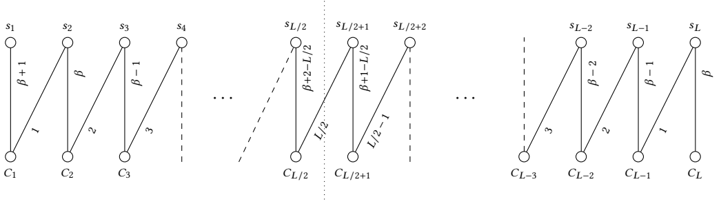
Fig. 2. Number of assignments of each type after each down-heavy phase. Each C_i has \beta + 2 clients for 1 \leq i \leq L/2 and \beta clients for L/2 + 1 \leq i \leq L . Each server has \beta + 1 clients assigned.
