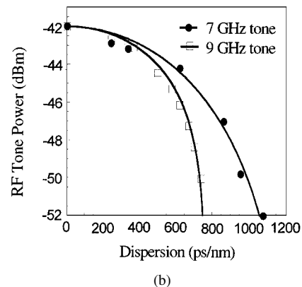
Fig. 3. (a) RF spectra of an 8-GHz tone in a 10-Gb/s transmission system at different amounts of accumulated dispersion. (b) RF fading due to dispersion for a 7- and 9-GHz tone. The solid lines represent the theoretical results and the points are experimental results.
