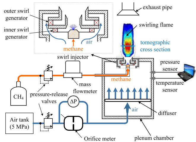
Fig. 2. Schematic of the experimental platform for swirl combustion.
