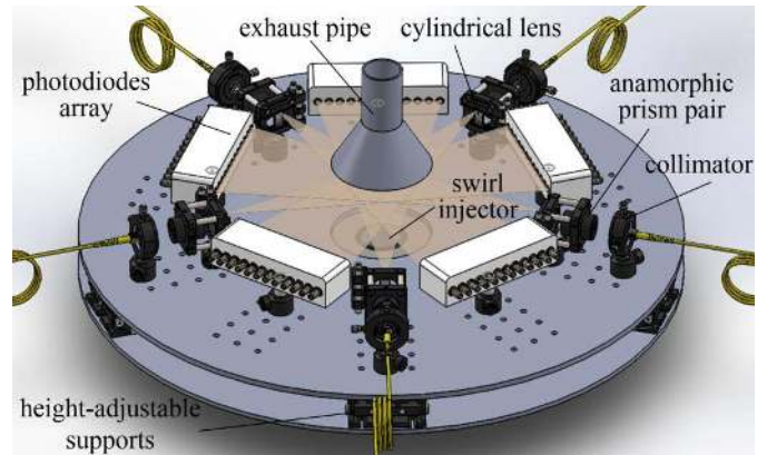
Fig. 5. Installation of the stationary TDLAS tomographic sensor above the nozzle of the model swirl injector.
