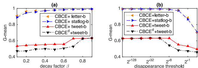
Fig. 12. Influence of (a) decay factor \beta and (b) disappearance threshold.
