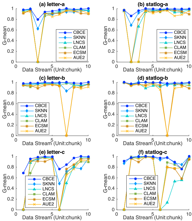
Fig. 8. G-means on the synthetic streams.
