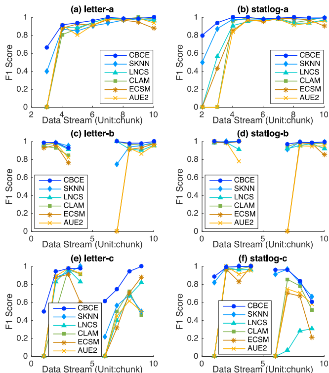
Fig. 7. F1 scores on the synthetic streams.
