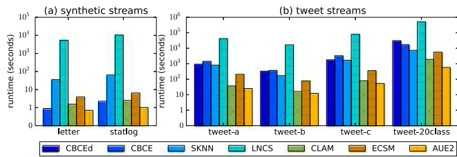
Fig. 11. Runtime of the compared approaches.
