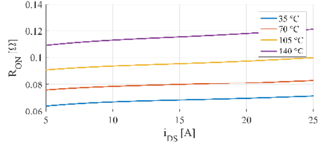
Fig. 13. R_{on} as a function of current.
