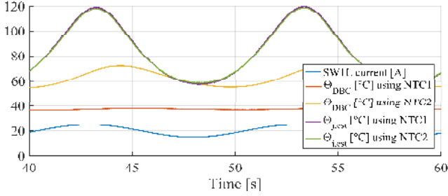
Fig. 20. Junction temperature estimation with sinusoidal current reference
