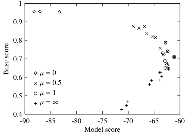
Figure 1: Scatter plot of 10-best unique translations of a single sentence obtained by forest rescoreing using various values of \mu in equation (11).
