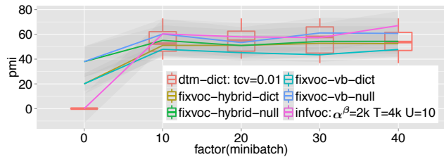
(a) de-news , S = 245 , K = 10 , \kappa = 0.6 and \tau_0 = 64
