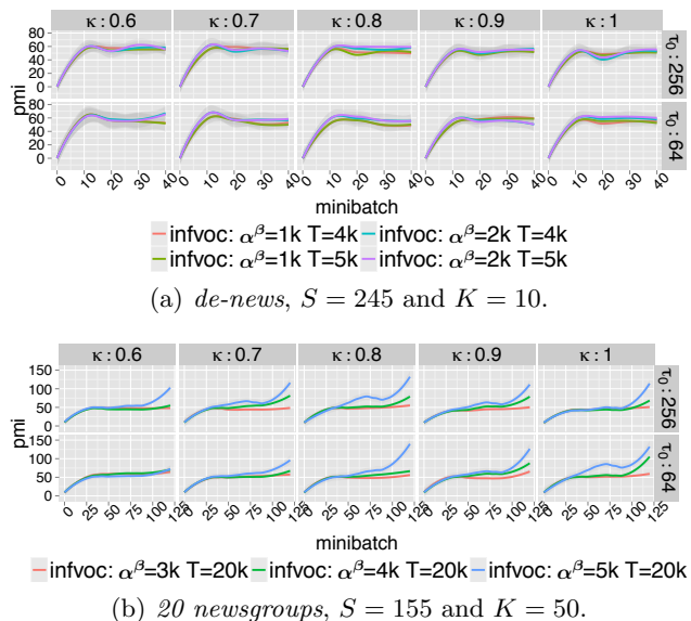
Figure 3. PMI score on two datasets with reordering delay U = 20 against different settings of decay factor \kappa and \tau_0 . A suitable choice of DP scale parameter \alpha^\beta increases the performance significantly. Learning parameters \kappa and \tau_0 jointly define the step decay. Larger step sizes promote better topic evolution.
