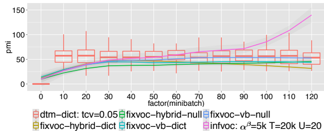
(b) 20 newsgroups , S = 155 , K = 50 , \kappa = 0.8 and \tau_0 = 64
