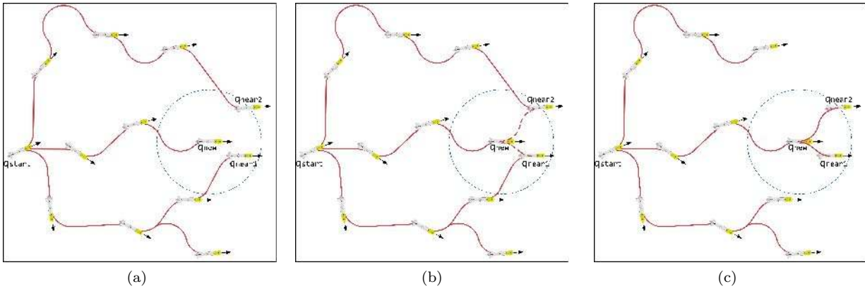
Figure 4: RRT* algorithm reconnection using Dubins curves as steering function. (a) Once a new configuration q_{new} has been obtained, (b) the RRT* algorithm checks if the nearest configurations to q_{new} can be reconnected. (c) If such a reconnection decreases the cost associated with the nearest configurations, new paths are created while discarding previous ones. This allows to progressively improve the solution path.
