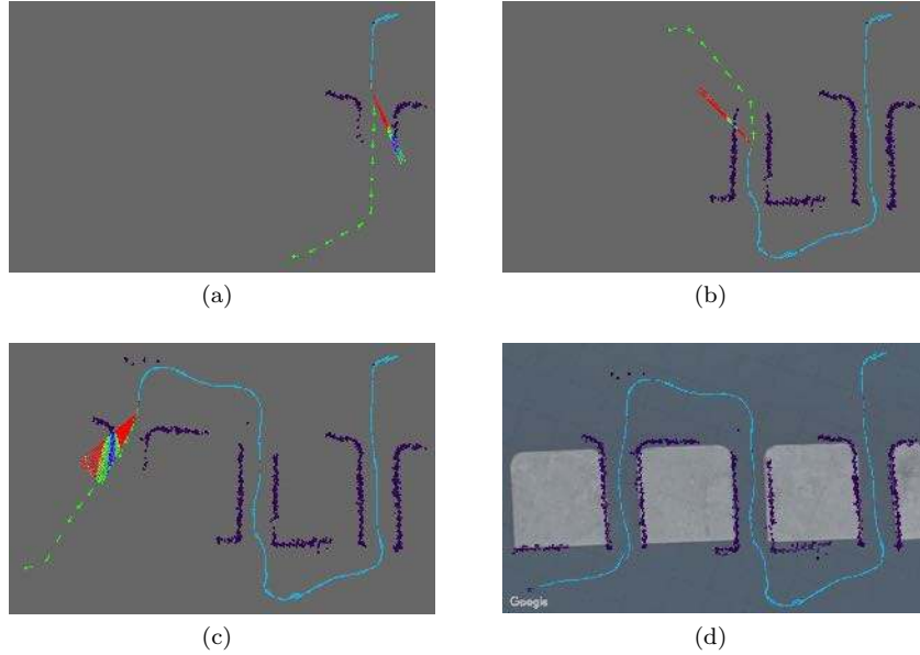
Figure 23: The Sparus II AUV used the motion planning framework to navigate through a breakwater structure without a preliminary map of the surroundings. (a), (b), (c) The mission required traversing the breakwater structure multiple times by solving successive start-to-goal queries. (d) The vehicle’s trajectory is drawn in light blue, while the map built with the imaging sonar data is presented in purple. This information is overlapped with a satellite image (Google Maps © 2017).
