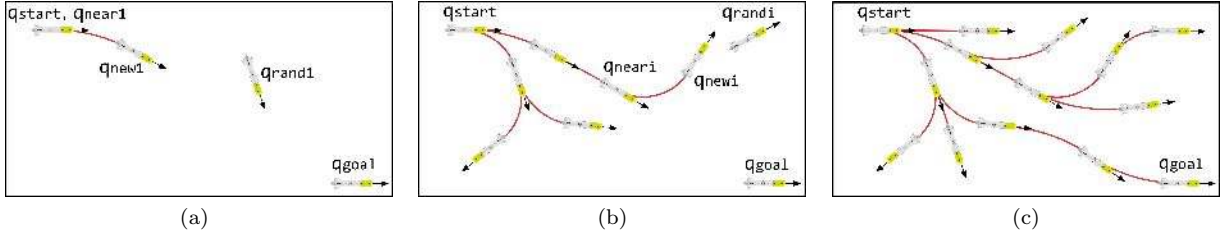
Figure 2: Tree expansion of an RRT algorithm that considers the differential constraints described by Equation (1). (a) Given the start and goal states, a first random sample is used to generate the first expansion of the tree ( q_{new} ). (b) The expansion i^{th} of the tree. (c) A feasible path has been found from the start to the goal state.
