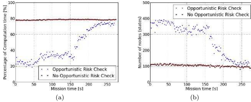
Figure 19: Incidence of Opportunistic State Checking approach when solving query presented in Fig. 18. (a) if configurations located in undiscovered areas are not assumed as safe, risk checking routines require almost 80% of computation time during the whole mission. Otherwise, the computation time will increase progressively as the environment is explored. (b) Consequently, if a high percentage of computing power is dedicated to risk checking, the number of tree nodes (states) will remain low during the whole mission, thus limiting the tree expansion and path quality.
