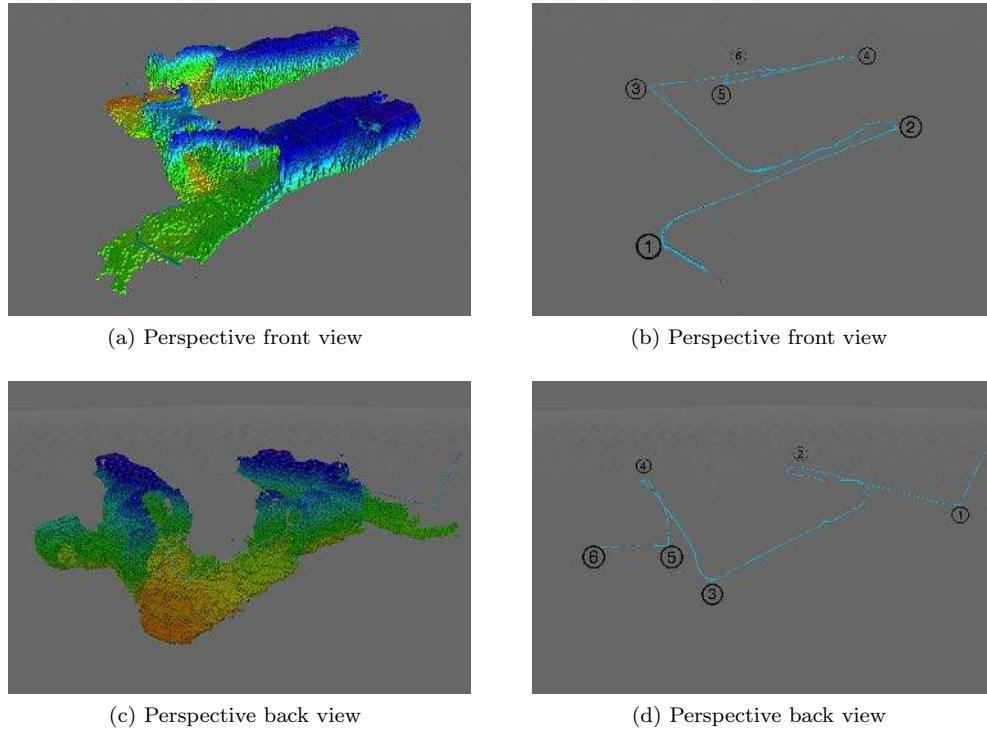
Figure 32: Simulated mission in the caves complex. The whole mission was composed of six start-to-goal queries that were executed consecutively.
