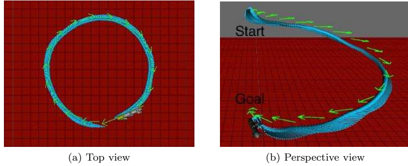
Figure 8: Start-to-goal query that is defined as q_{start} = [x_0, y_0, z_0, \psi_0] and q_{goal} = [x_0, y_0, z_0 + depth, \psi_0] . The AUV is assumed to navigate at a constant surge speed v , and a descending speed up to d_{max} . The solution path (in green) is calculated with an RRT* that uses the extended Dubins curves, which incorporate the vehicle's 3D motion capabilities. The simulated Sparus II successfully describes a helical trajectory (in light blue) that follows the calculated path.
