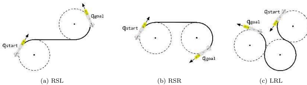
Figure 3: Examples of Dubins curves
