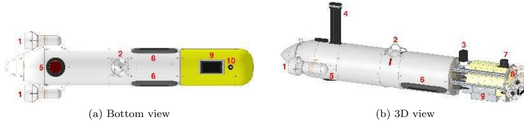
Figure 33: Sparus II AUV: bottom and 3D views. Different hardware parts can be observed, including the thrusters (1,2), the acoustic modem (3), the Wi-Fi and GPS (4), as well as interoceptive and exteroceptive sensors such as the DVL (5), side-scan sonar (6), mechanically-scanning imaging sonar (7), single-beam echosounders (8), multibeam sonar (9), and an optical camera (10).
