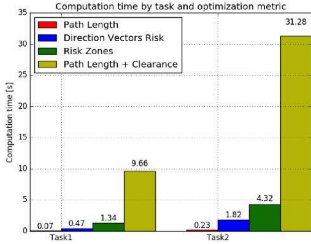
Figure 16: Average computation time, over 100 runs, required to solve Task1 and Task2 (Fig. 15) using different approaches to include risk of the path as the optimization criterion.
