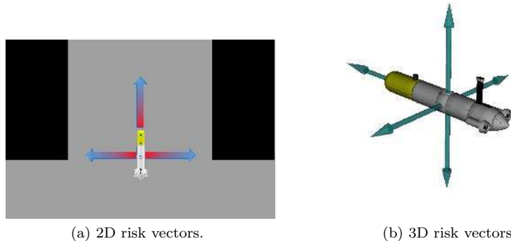
Figure 13: (a) Sparus II AUV navigating between two obstacles (black). An example of the risk vectors, and how the risk decreases as moves away from the vehicle can be observed (red means high risk, while blue low risk). (a) Extension of risk vectors for 3D motions.
