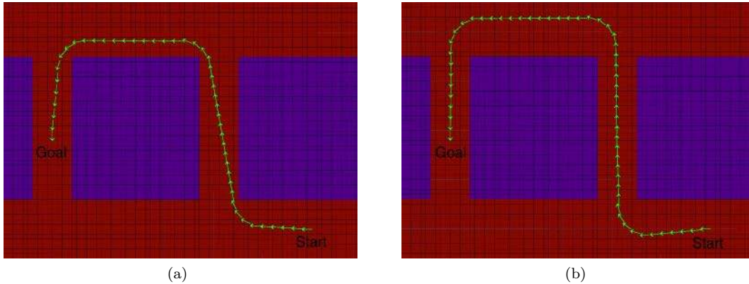
Figure 12: (a) RRT* expansion for a start-to-goal query using Dubins curves with path length as cost criterion. (b) RRT* expansion with risk zones cost criterion. It is worth noting that the resulting path is far from corners in turning maneuvers and attempts to stay in the middle of the corridor when navigating between two obstacles.
