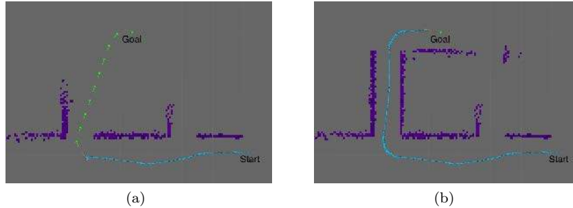
Figure 18: A simulated Sparus II in an equivalent virtual scenario of the breakwater structure. The vehicle starts a mission by submerging to a specified depth. It then maps and solves a start-to-goal query simultaneously. (a) Equipped with a scanning profiler, it incrementally builds a representation of the environment, while continuously reshaping the solution path, (b) to finally approach to the specified goal configuration.
