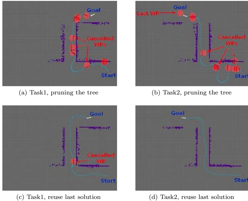
Figure 20: Comparison of the pruning tree scheme and the reuse of the last best known solution when solving start-to-goal queries with the pruning-tree scheme and the reuse of the last best known solution approaches. Cancelled waypoints (WPs) are presented as circles in red, and correspond to WPs that may lead the vehicle to a collision, thus requiring the path to be completely replanned.
