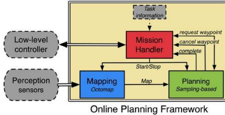
Figure 10: Framework for online AUV motion planning.
