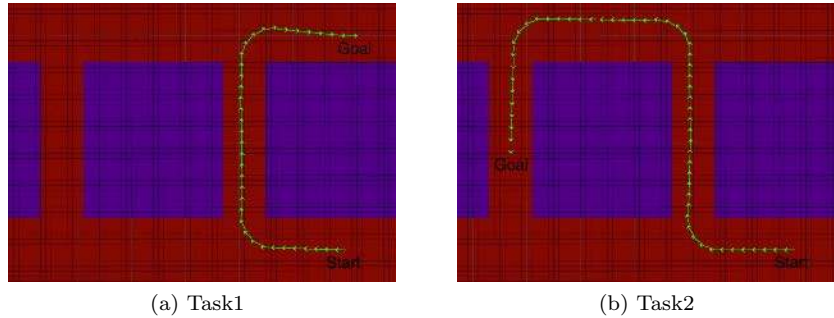
Figure 15: Solutions to start-to-goal queries using an RRT* algorithm with Dubins curves and risk functions. The solution paths maintain a safe distance from nearby obstacles (areas in purple).
