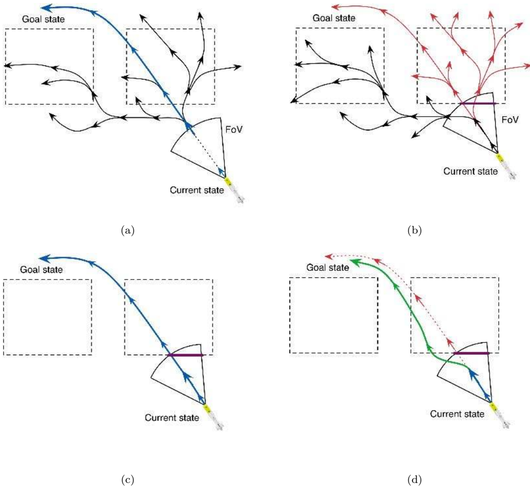
Figure 14: A test scenario in which a vehicle simultaneously maps and plans collision-free paths in an unexplored environment. The vehicle is assumed to be equipped with a forward-looking range sensor of limited FoV to navigate in an environment that contains a series of obstacles, which are separated by gaps. The task consists in a start-to-goal query that requires navigating from one side of the obstacles to the other. (a) During the first part of the task when no obstacle has been detected, the solution path corresponds to the shortest one from the vehicle's current state to the goal state (see nodes and branches in blue). (b) Once an obstacle is inside the vehicle's sensor FoV (in purple), different strategies could be used to guarantee that the solution path is still valid. With the tree-pruning strategy the tree is rechecked for collision. Nodes and edges that are in collision, as well as the subtrees attached to them, are discarded. This strategy may occasionally lead to loss of valuable information about reaching the goal, even if only part of the previous solution was affected (see parts of the tree in red). (c) An alternative is keeping the last best known solution (in blue), and then reusing it as an starting point in the next planning cycle, (d) which will discard the affected parts, while attempting to reconnect to other valid parts of the previous solution (in green).
