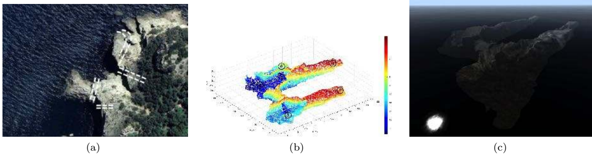
Figure 29: (a) The underwater caves complex “Coves de Cala Viuda” is located in the L’Escala, Spain (Lat: 42.10388, Lon: 3.18255). It consists of three single-branch caves and several tunnels. Their approximate positions are marked with dotted white lines. (b) Meshed map using the SNDC algorithm (Campos et al., 2013). Over the map, the approximate locations of six different goals have been marked in black. Images credit: Mallios et al. 2015 (Mallios et al., 2015; Mallios et al., 2017). (c) Mesh map added into UWSim as a simulation environment.
