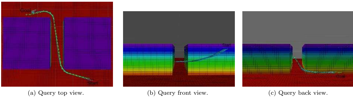
Figure 9: Virtual breakwater structure composed of two obstacles that create a narrow passage. The solution path (in green) is calculated by an RRT* that uses the extended Dubins curves approach. A simulated Sparus II AUV describes a trajectory (in light blue), which does not differ significantly from the one calculated, even when conducting turning maneuvers.
