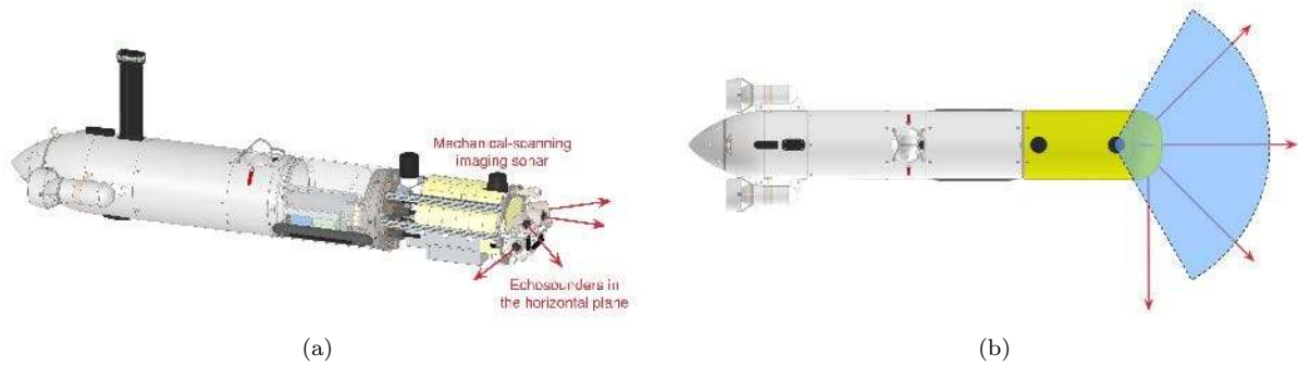
Figure 22: Exteroceptive sensors configuration for the Sparus II AUV to conduct autonomous missions in the breakwater structure. (a) The vehicle was equipped with four echosounders and one mechanical-scanning imaging sonar, all of them pointing in the horizontal plane. (b) Top view, echosounders beams direction and imaging sonar scan sector.
