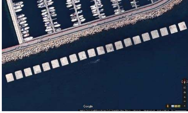
Figure 5: Breakwater structure composed of a series of concrete blocks (14.5m long and 12m width, separated by a four-meter gap) in Sant Feliu de Guíxols in (Spain). Image credit: Map data ©2017 Google.
