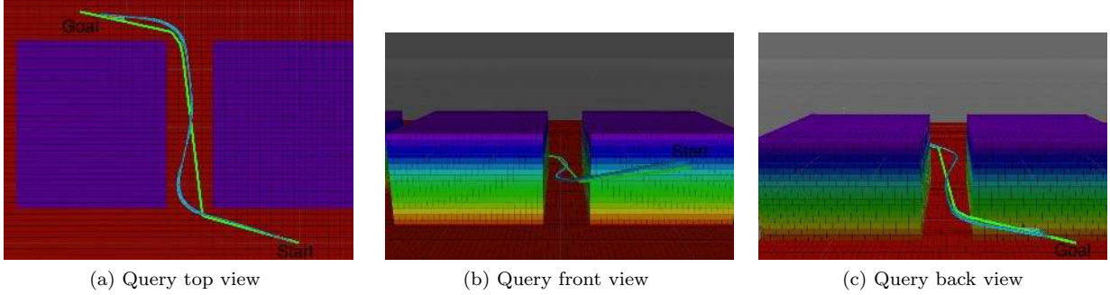
Figure 6: Virtual breakwater structure composed of two obstacles that create a narrow passage, where a start-to-goal query is defined as q_{start} = [x_0, y_0, z_0] and q_{goal} = [x_1, y_1, z_1] . The solution path (in green) is calculated only taking into account geometric constraints. A simulated Sparus II AUV attempted to follow the path, however the resulting trajectory (in light blue) differs from the one calculated, thus leading to risky situations when conducting turning maneuvers.
