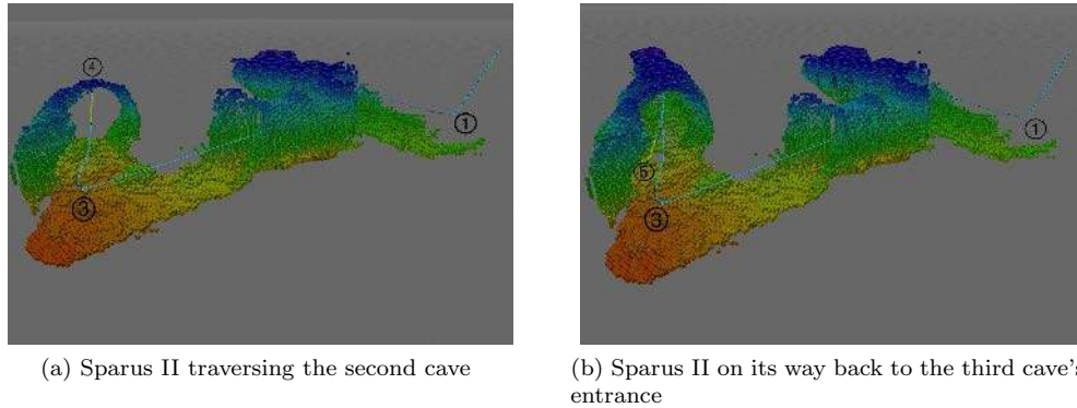
Figure 31: Simulated mission in the caves complex. (a) The fourth start-to-goal query required the vehicle to navigate through the second single-branch cave. (b) The fifth query was defined to guide the vehicle close to a third cave's entrance. This required the planner to find a way out of the cave. In both images, the vehicle's trajectory appears in light blue.
