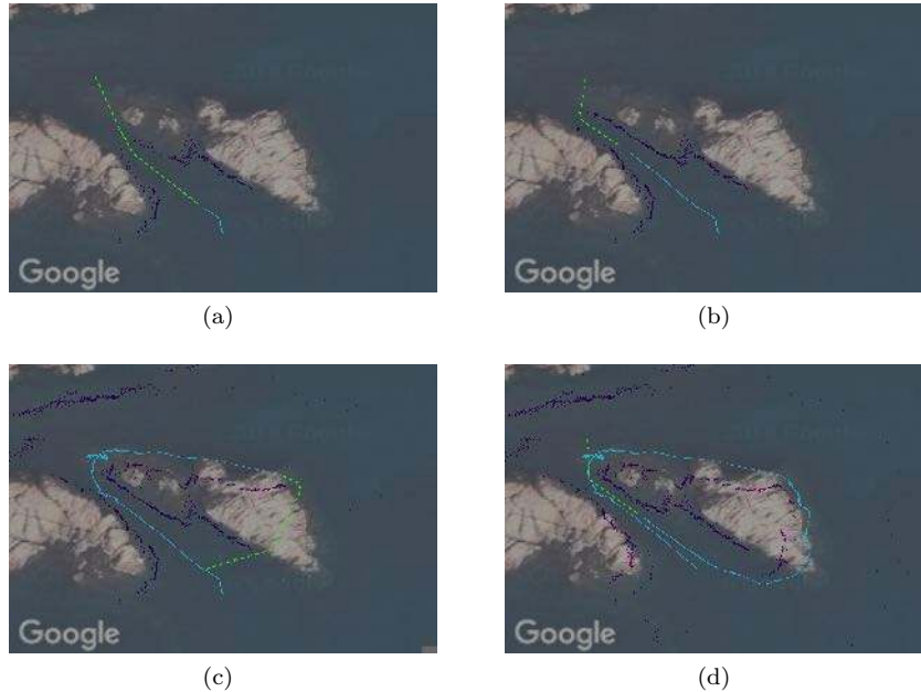
Figure 26: The Sparus II AUV used the motion planning framework to navigate through an underwater canyon without a preliminary map of the surroundings. (a), (b) The first start-to-goal query required the Sparus II traversing an underwater canyon. (c) For the second query, the vehicle circumnavigated the outer rock. (d) The AUV partially repeated the first start-to-goal query in order to close the loop and to obtain overlapped images. Vehicle’s trajectory and Octomap overlap a satellite image (Map data ©2017 Google).
