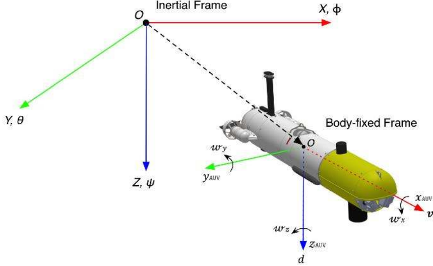
Figure 1: Perspective view of the Sparus II AUV, including the inertial and body-fixed frames, and the 6D vehicle's state and control variables
