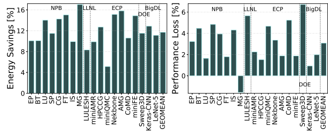
Fig. 6: Energy savings and the resulting slowdowns on a single CascadeLake node with respect to the baseline power management scheme (Section 4.5).
