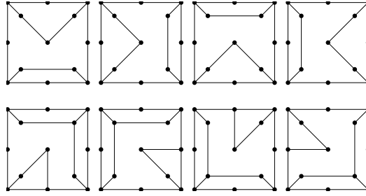
FIG. 2.1. Any deterministic memoryless algorithm is defeated by at least one of these graphs.
