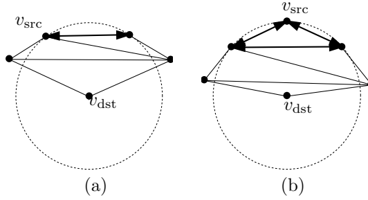
FIG. 2.2. Triangulations that defeat the greedy routing algorithm.
