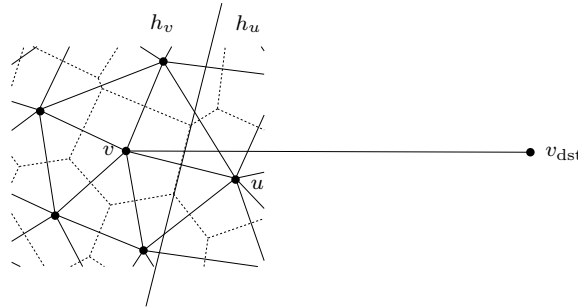
FIG. 2.3. The proof of Theorem 2.1.
