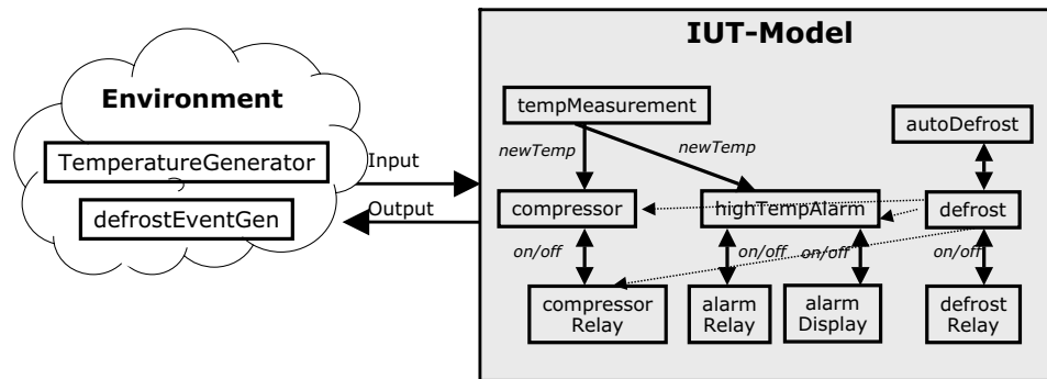
Fig. 10. Main timed automata components in model
