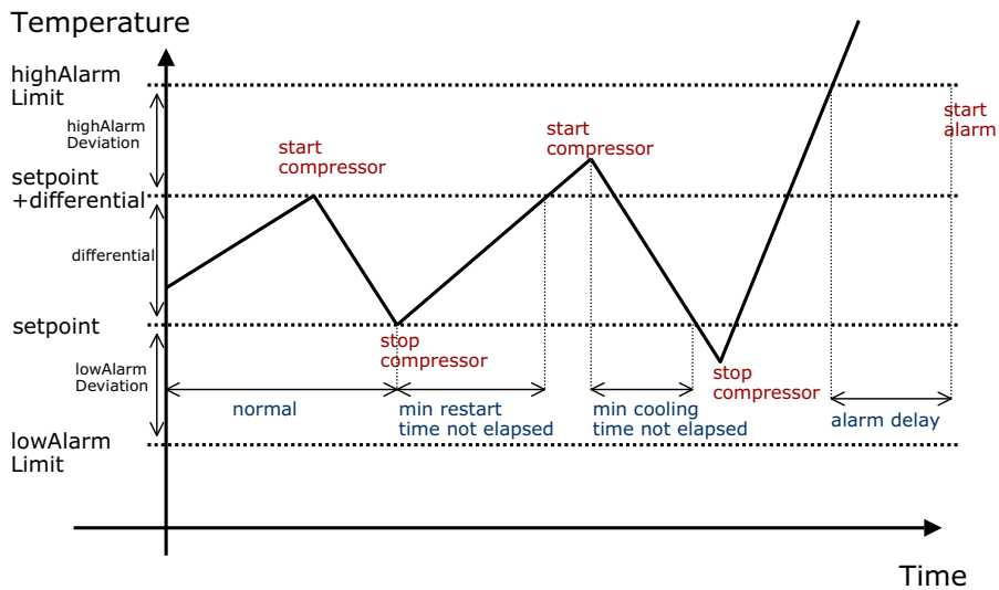
Fig. 9. Main Control Objective of an EKC is to maintain temperature within bounds.
