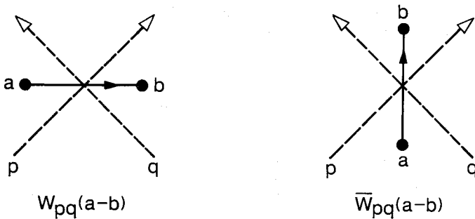
Fig. 7. Boltzmann weights for the chiral Potts model.
