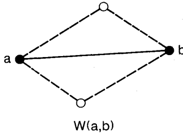
Fig. 5. Mapping from spin model to IRF model, adding trivial spins on dual lattice.
