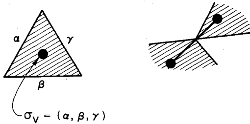
Fig. 4. Mapping from vertex model to spin model.
