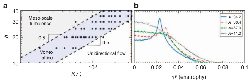
Figure 2 | Competing length scales control the transition to active turbulence. (a) Phase-space of control parameters corresponding to the vortex-lattice state. The slope of 0.5 at the boundaries of the vortex-lattice state shows that the emergence of vortex lattice is controlled by two competing length scales: the channel height h and the activity length scale \sqrt{K/\zeta} . (b) Transition from the vortex-lattice state to active turbulence is characterized by the channel-averaged enstrophy \epsilon distribution for increasing values of activity number A = \sqrt{\zeta h^2/K} .
