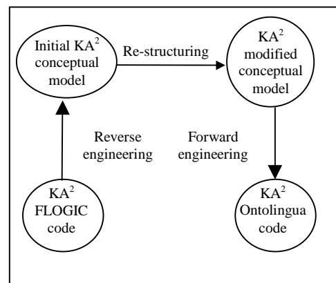
Figure 2. Ontological Reengineering Process of the (KA) 2 Ontology.
