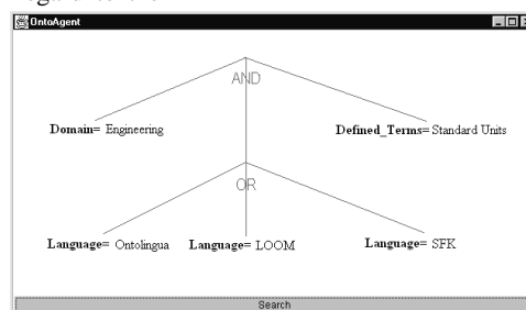
Figure 8. (ONTO) 2 Agent is asked to provide all the ontologies in the engineering domain, written in Ontolingua, LOOM or SFK, with Standard Units as a defined term, using a query expressed by means of an AND/OR tree.
