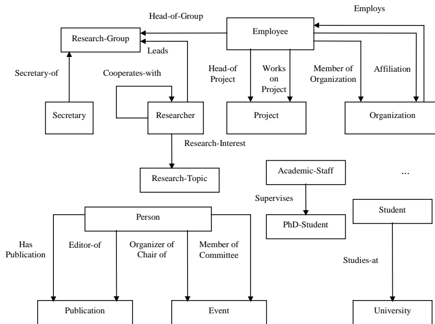
Figure 3. Concept Classification Tree in (KA) 2 .
