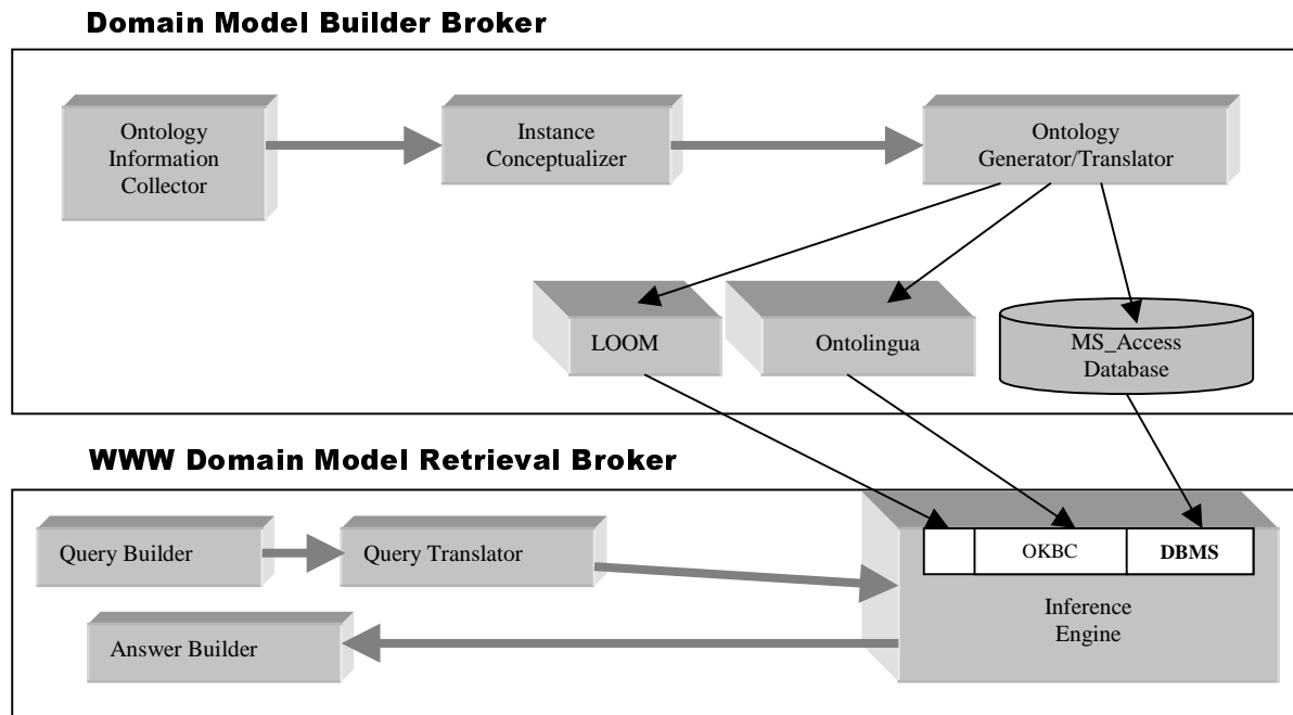
Figure 6. OntoAgent architecture.
