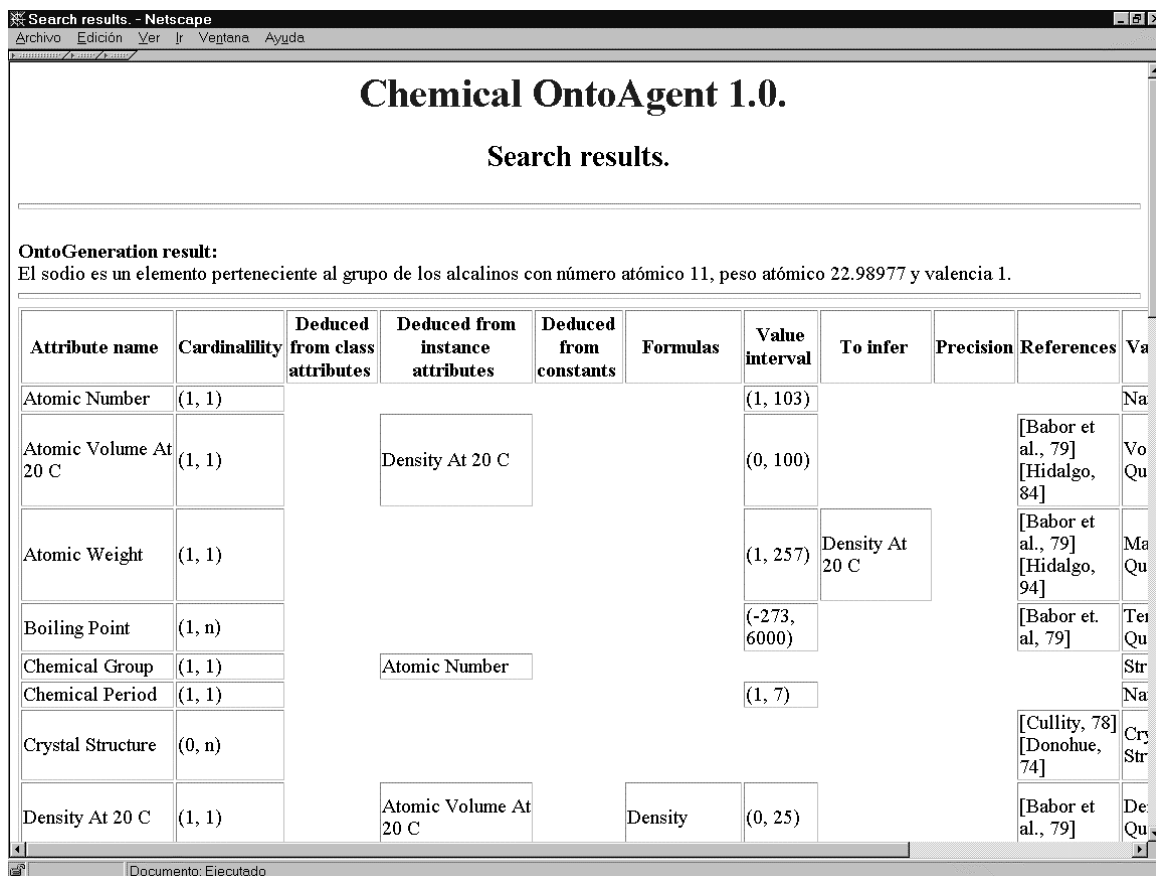
Figure 9. Search results in natural language and in tabular form. Sodium definition: Sodium is an element that belongs to the alkaly metal group and has an atomic number of 11, an atomic weight of 22.98977 and a valency of 1. The table also shows the Chemicals instance attributes table.
