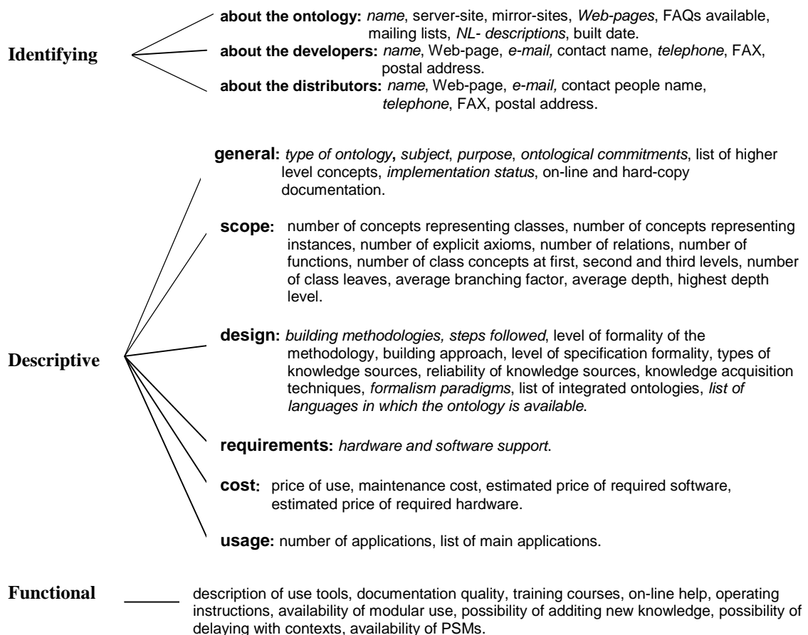
Figure 1. Feature taxonomy.
