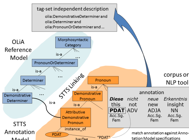
Figure 2: Interpreting annotations in terms of the OLiA Reference Model
