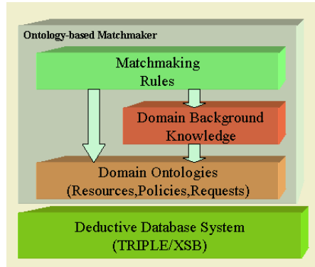
Fig. 3. Ontology-based Matchmaker
