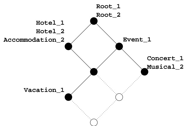
Figure 4: The pruned concept lattice
