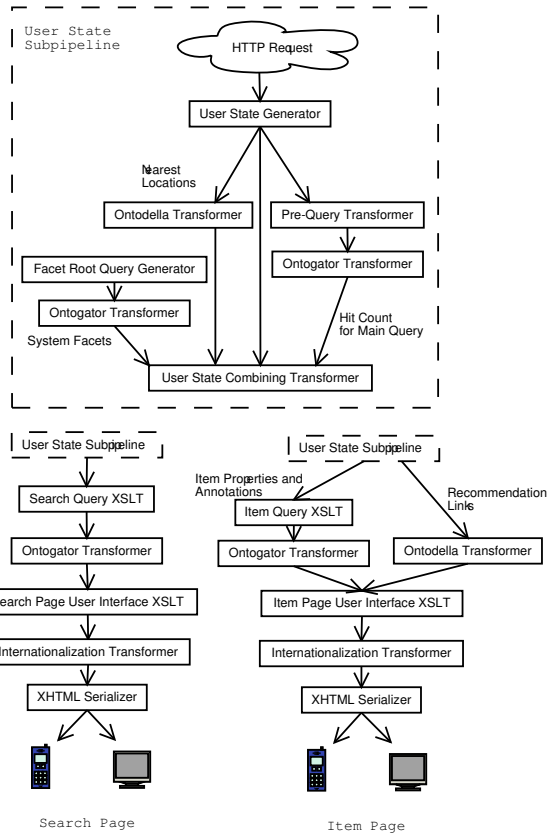
Fig. 8. Two Cocoon pipelines used in ONTOVIEWS.
