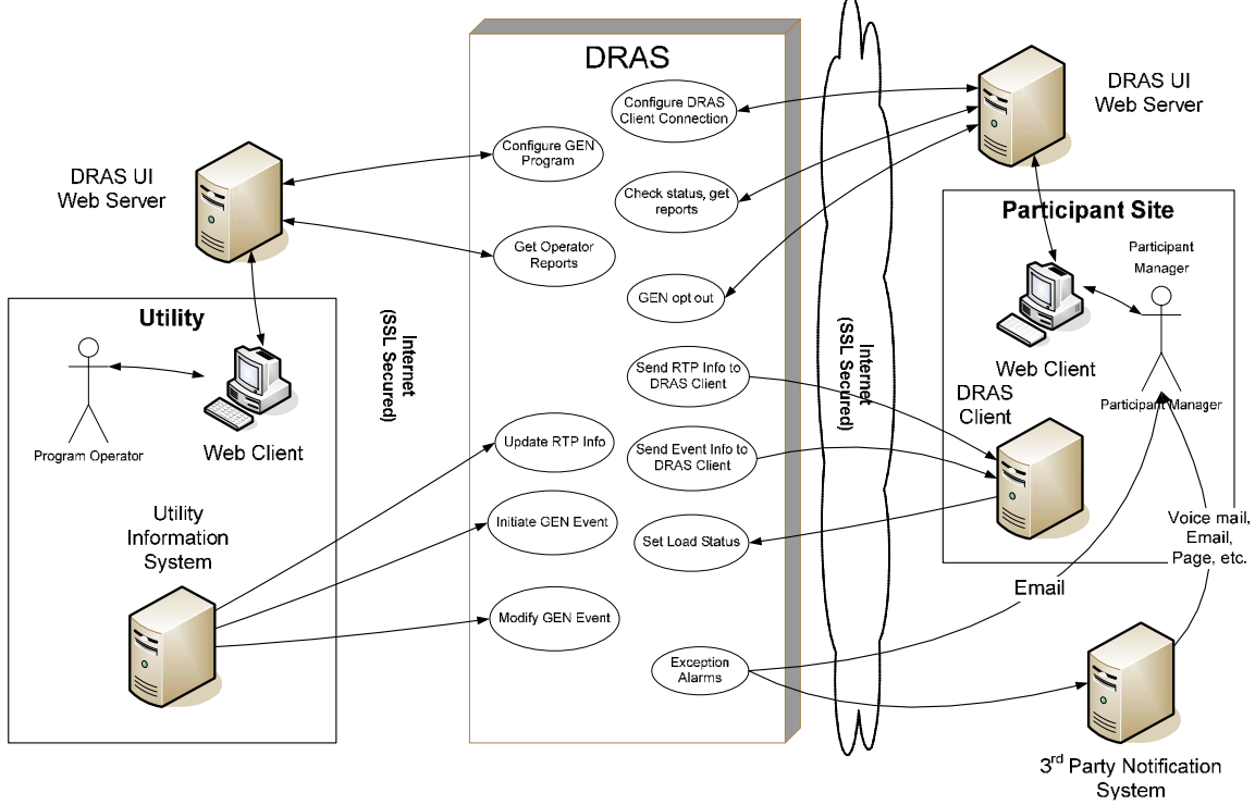
Figure 4. General Automated Events Architecture with Standalone DRAS
