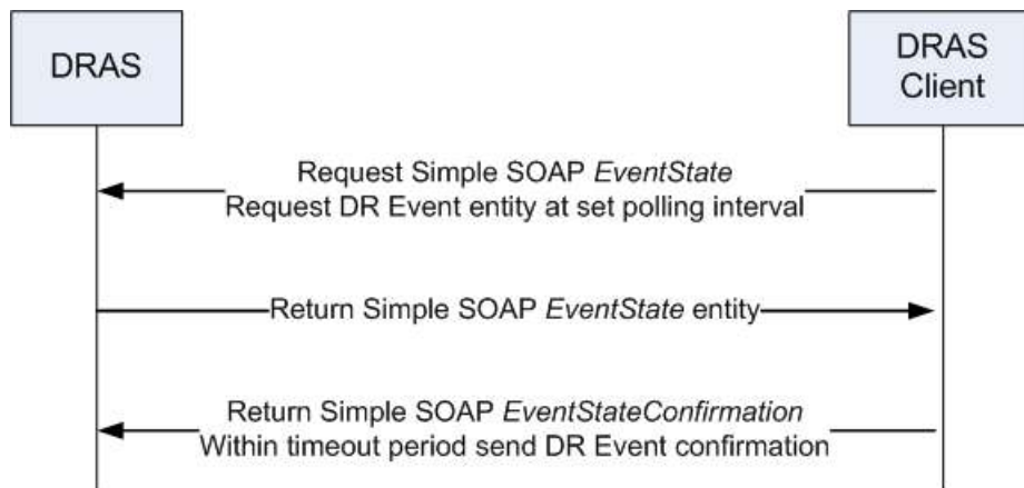
Figure 42. Simple SOAP PULL Model Sequence Diagram
