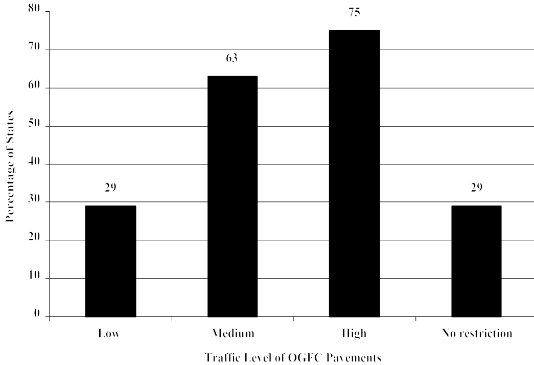
Figure 5. Traffic Level of Pavements on Which OGFC is Used
