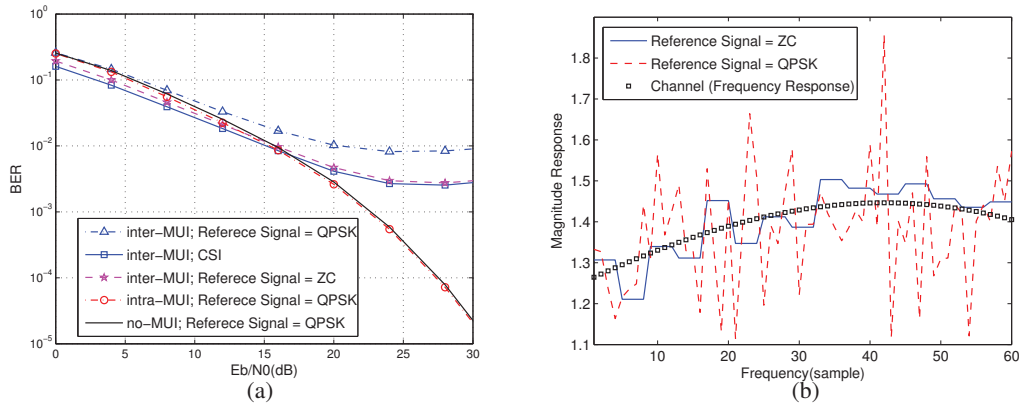
Fig. 4. Uplink transmission (Turbo Code off): (a) intra-MUI vs. inter-MUI and (b) channel estimation.
