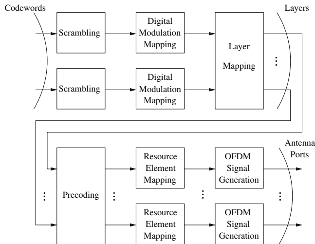
Fig. 1. Transmission scheme for the downlink connection.
