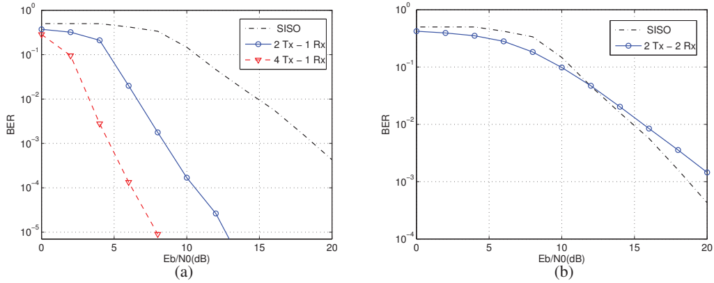
Fig. 3. Downlink transmission (Turbo Code on): (a) diversity transmission and (b) spatial multiplexing.
