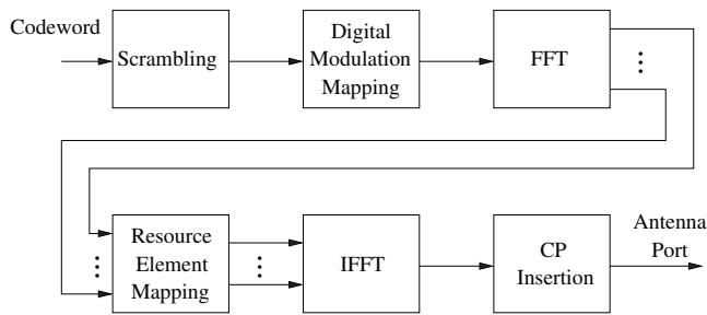
Fig. 2. Transmission scheme for the uplink connection.
