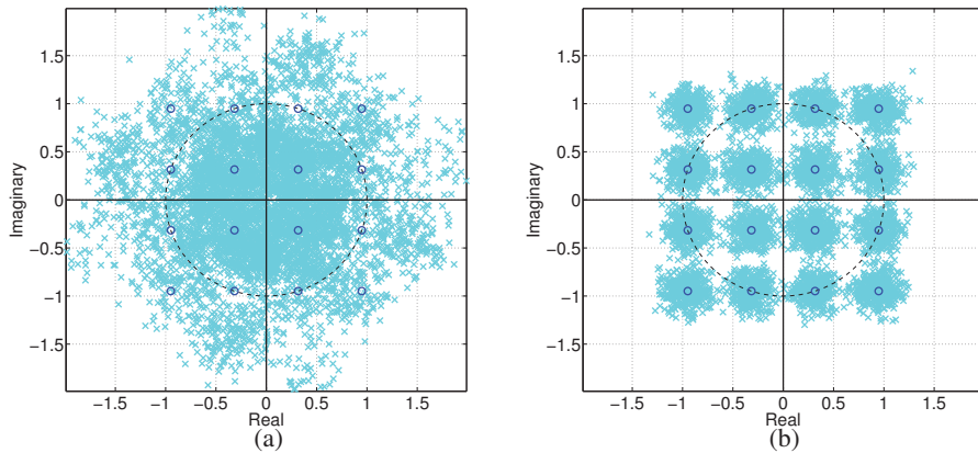
Fig. 5. Received symbols in uplink transmission with E_b/N_0 = 30 dB: (a) before equalization and (b) after equalization.
