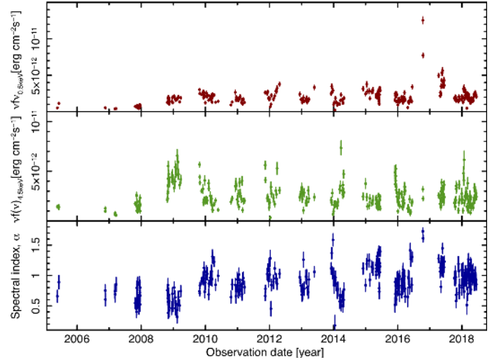
Fig. 8. v f(\nu) flux at 0.5, 4.5 keV and the power-law energy spectral index of the blazar OJ 287 are plotted against observation date. Many differences in the top and middle panels are clearly visible; in particular, the X-ray flares occur in different periods in the soft (0.5 keV) and hard (4.5 keV) parts of the X-ray spectrum.
